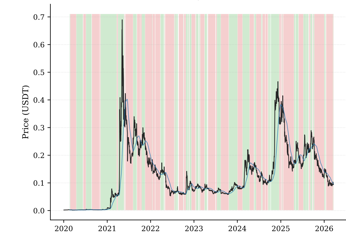
DOGE/USDT
