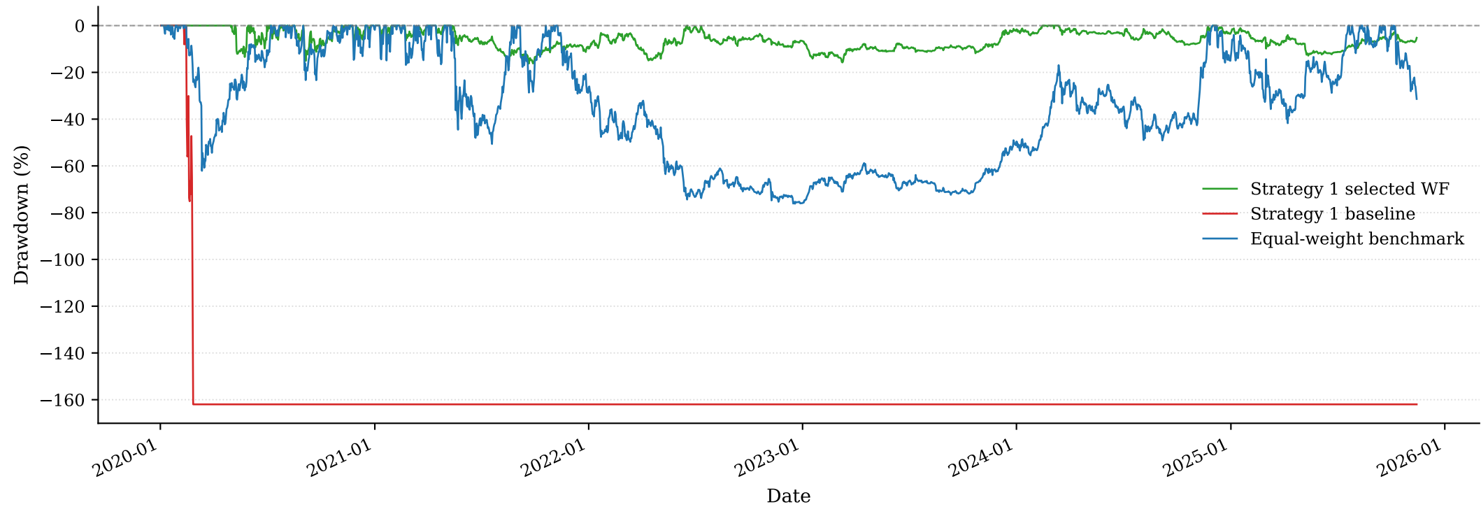
Strategy 1 development sample: underwater / drawdown profile
