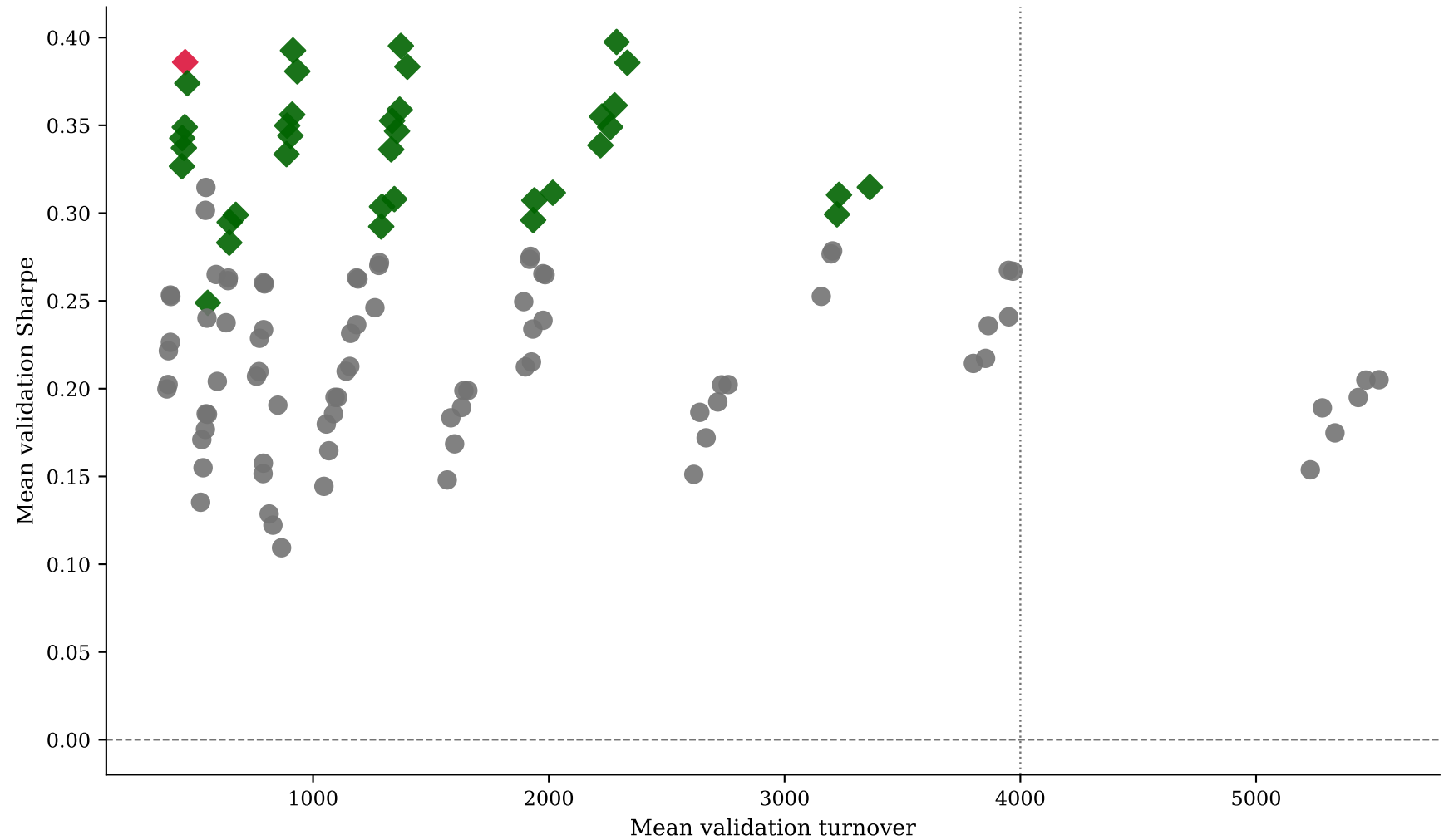
Strategy 1 validation Sharpe vs turnover
