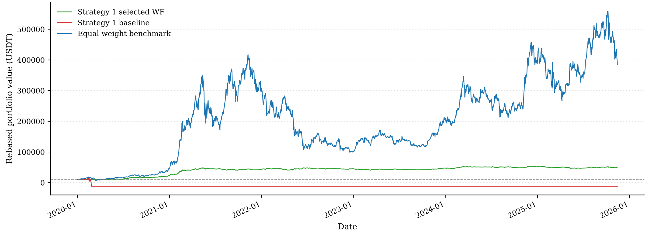
Strategy 1 development sample: rebased wealth comparison
