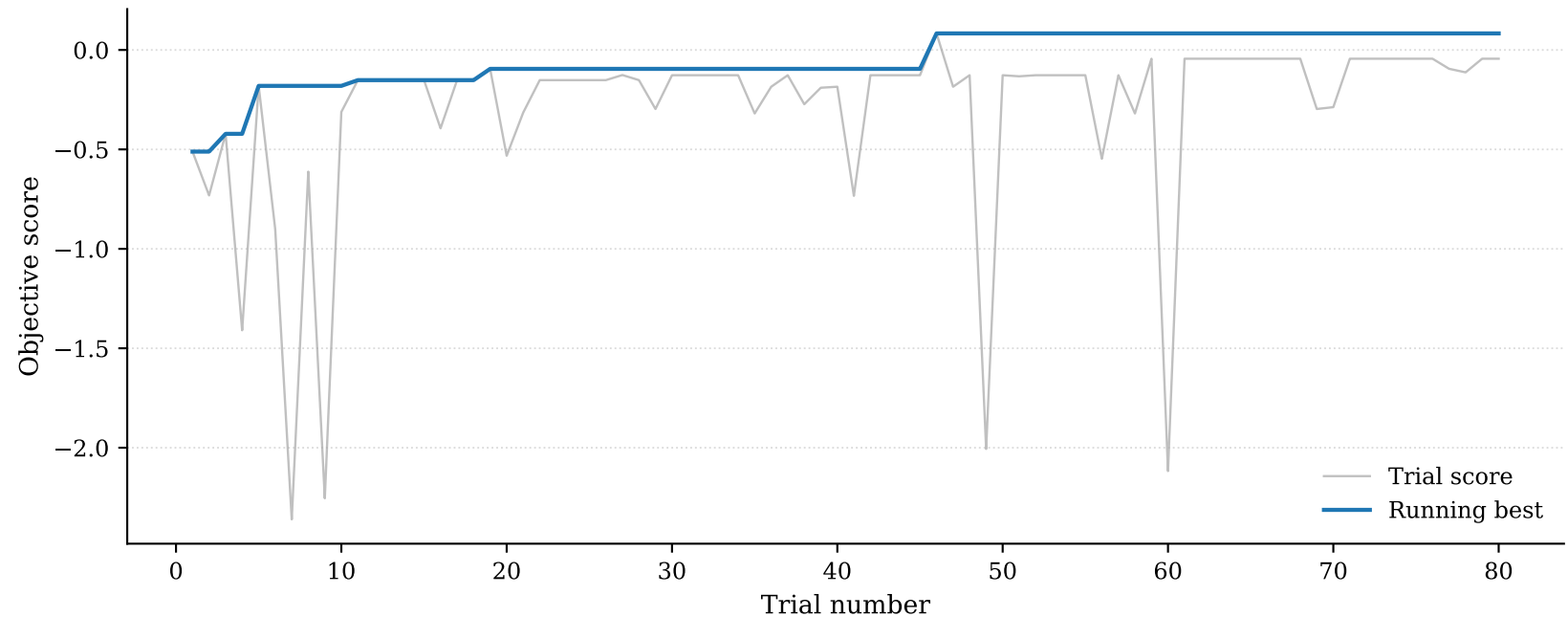
Strategy 2 Optuna optimisation history
