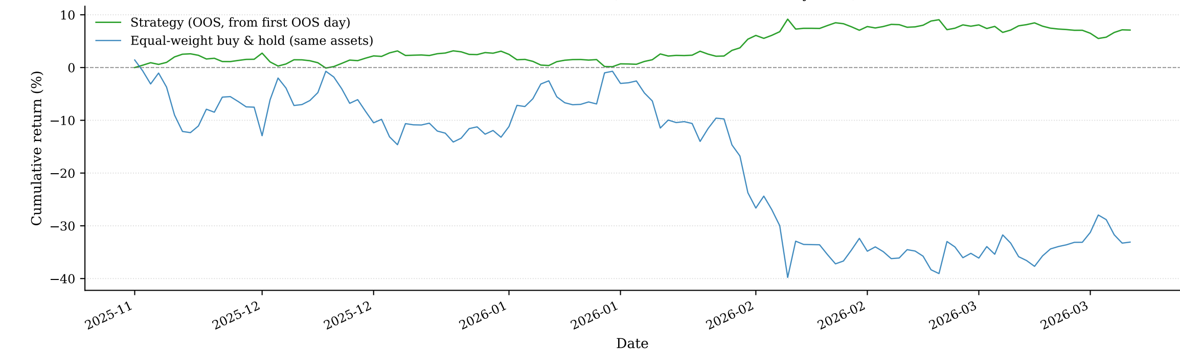
Final OOS cumulative return (normalized to first OOS day = 0%)
