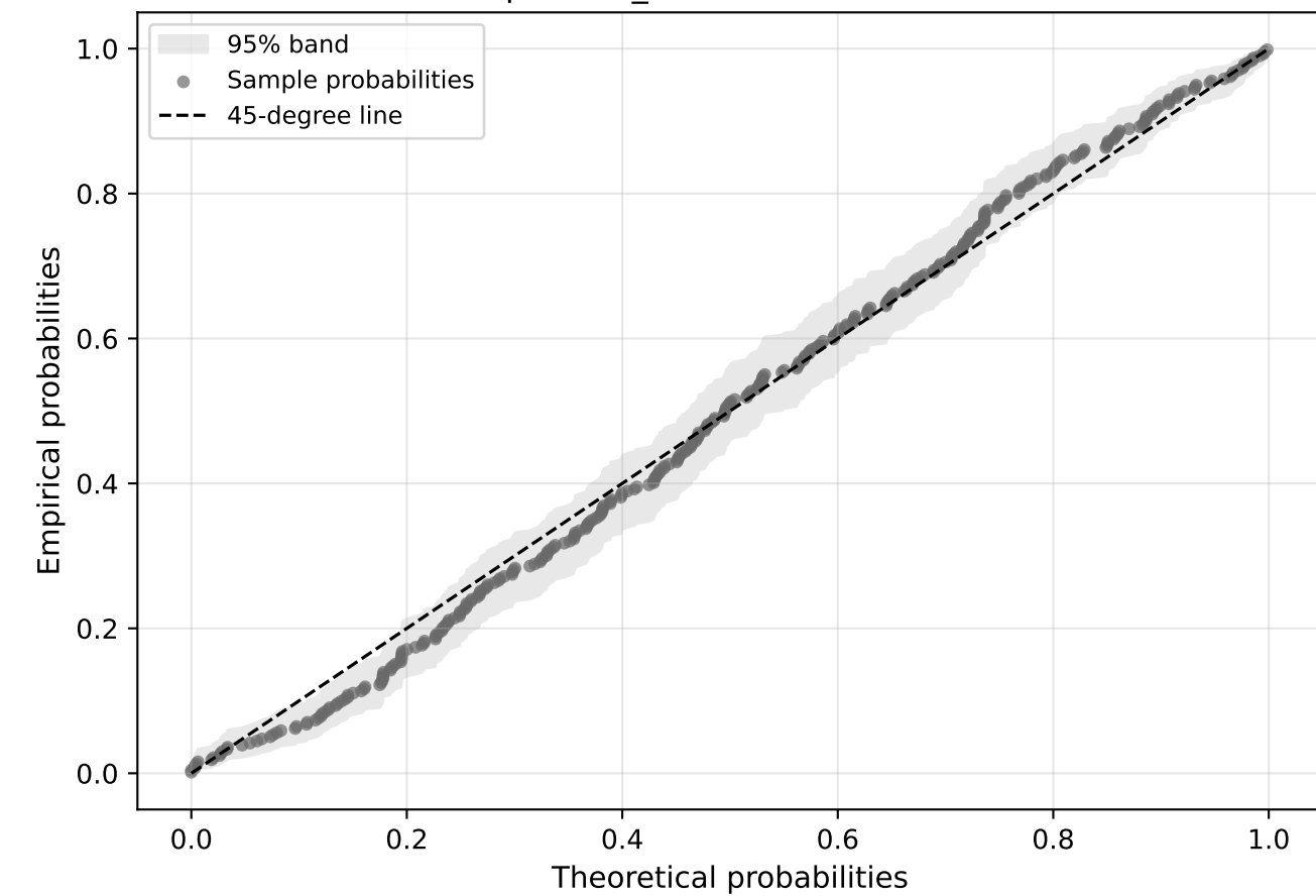
P-P plot of r_{\text{true}} vs fitted Gaussian
