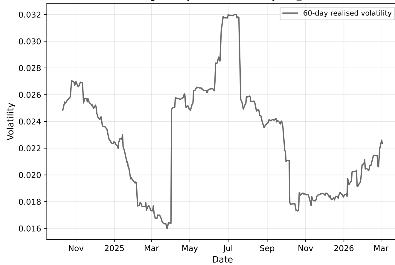
Rolling 60-day realised volatility of r_{\text{true}}
