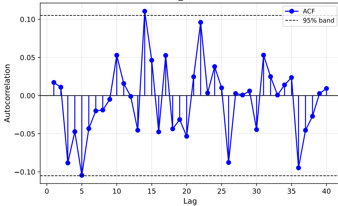
ACF of z_t (Composite LSTM)
