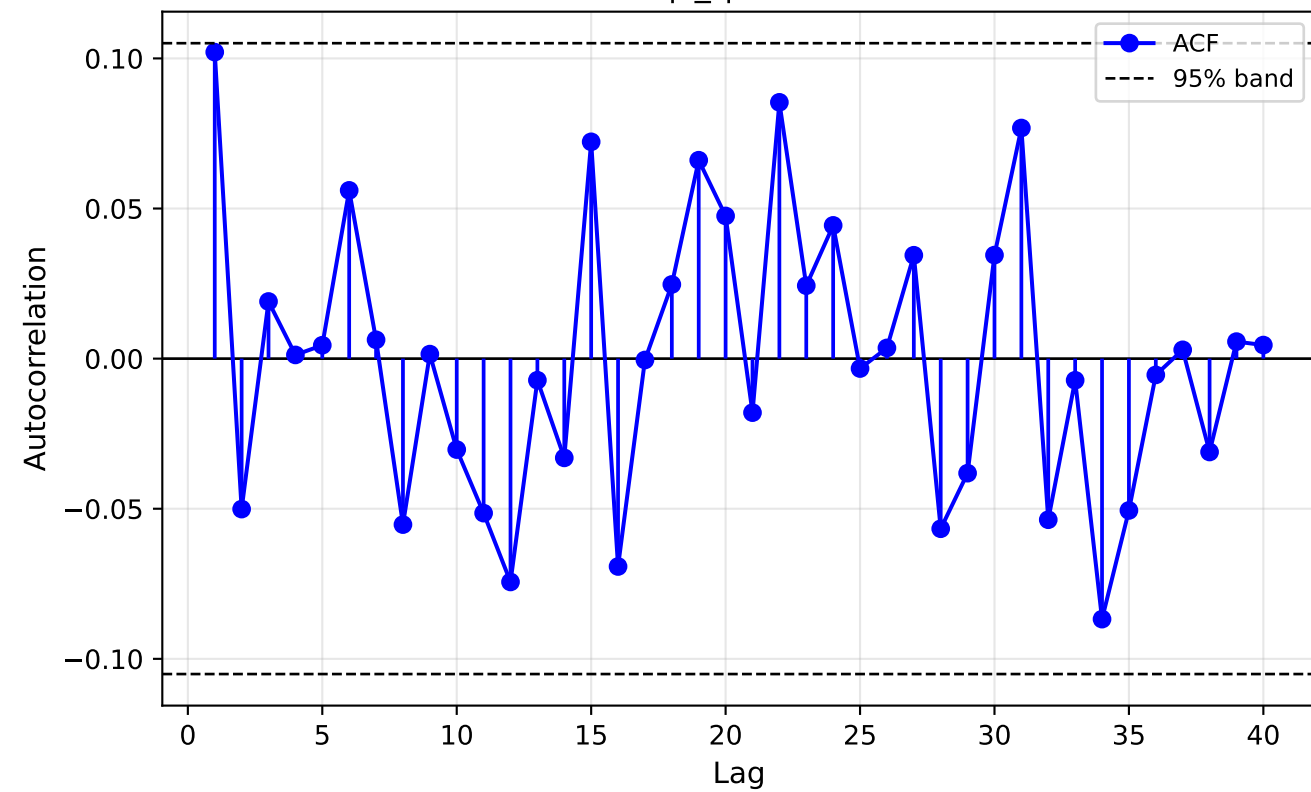
ACF of |z_t| (Composite LSTM)
