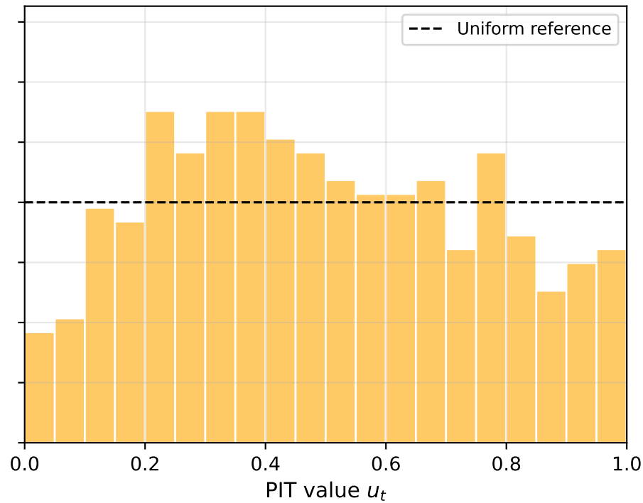
Composite LSTM
