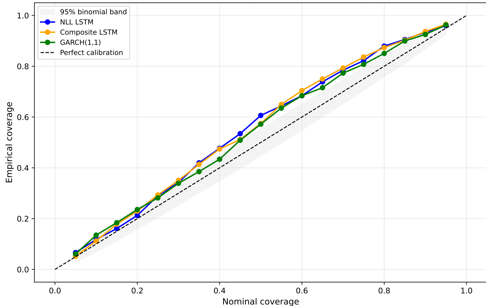
Calibration curve: empirical vs nominal coverage
