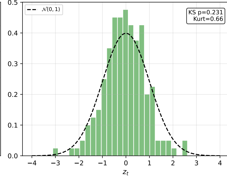
GARCH(1,1) Low-volatility (n=174)
