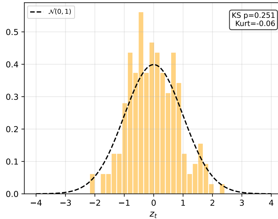
Composite LSTM Low-volatility (n=174)
