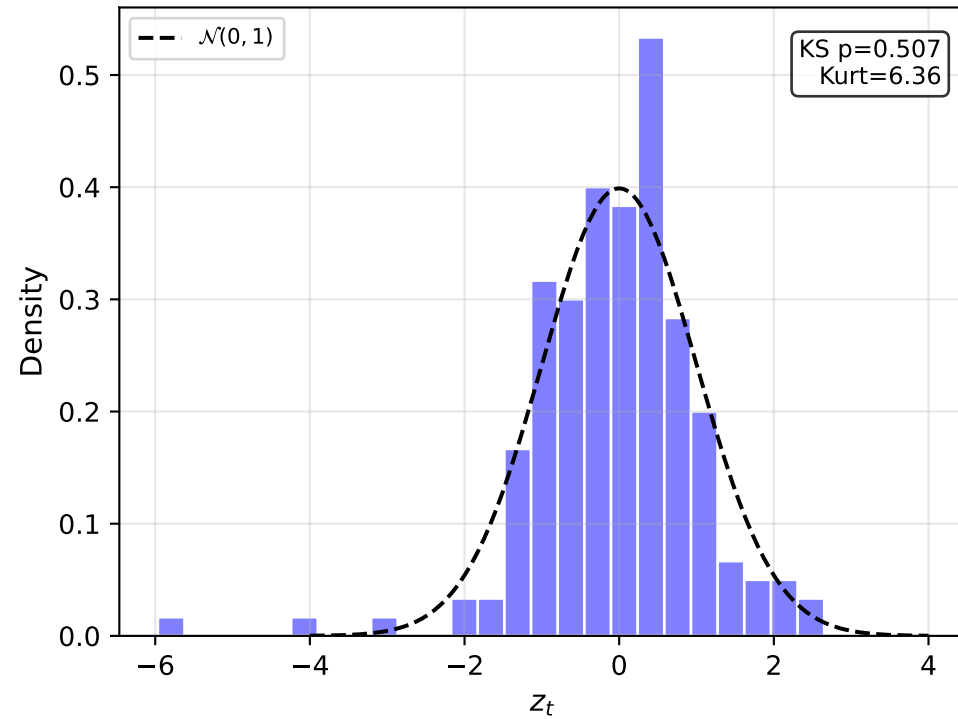
NLL LSTM Low-volatility (n=174)
