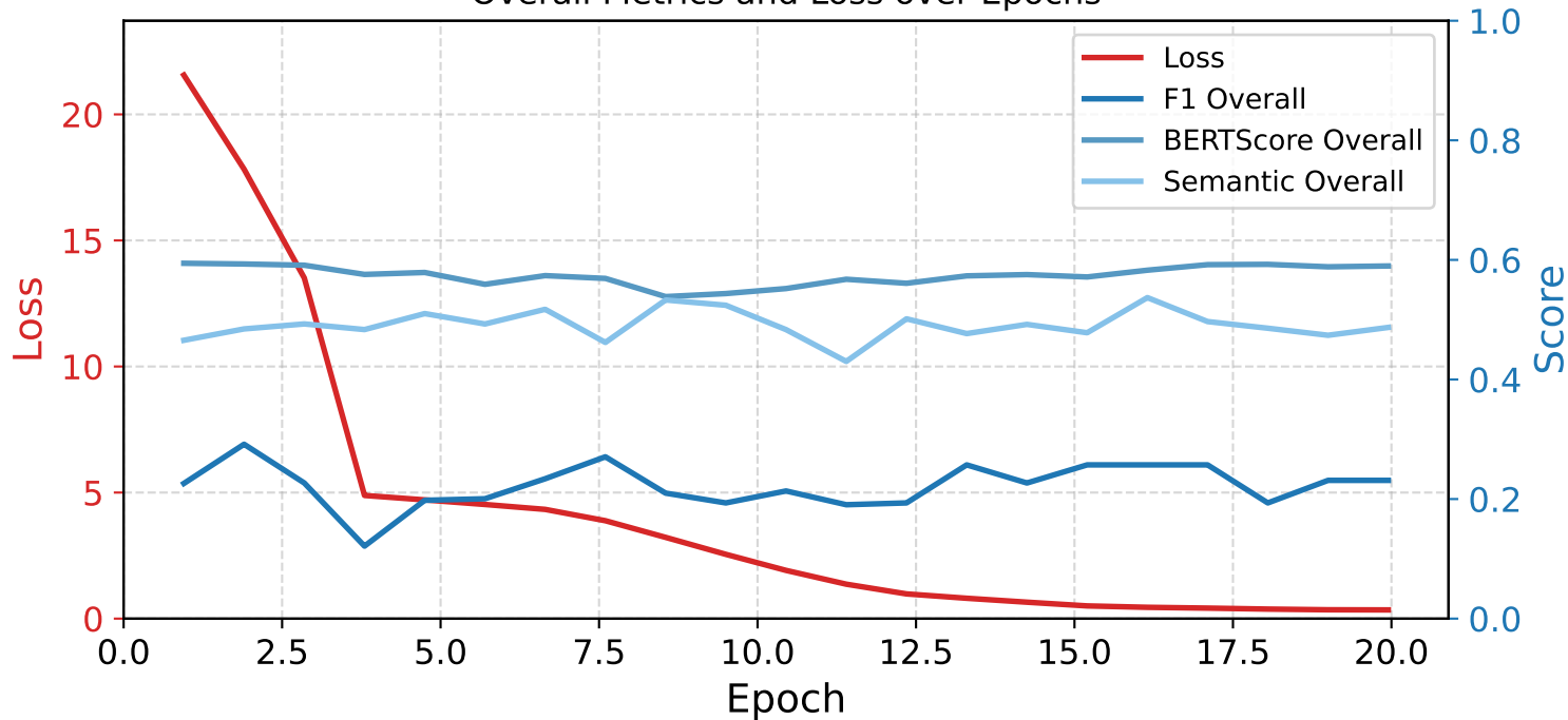
Overall Metrics and Loss over Epochs
