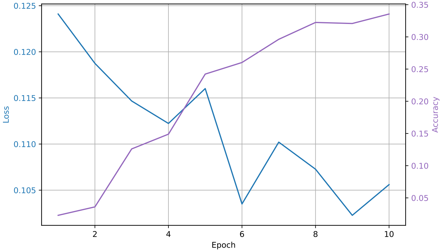
Training Metrics
