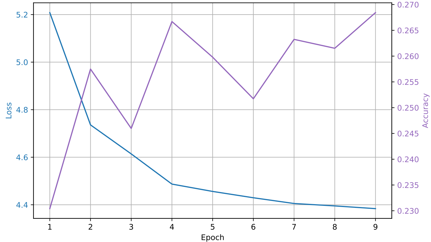
Training Metrics
