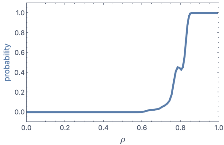
Probability of false-positive responses to random queries, as a function of memory density \rho . This simulation uses heteroassociations with N = 1,000 and P = 10 .
