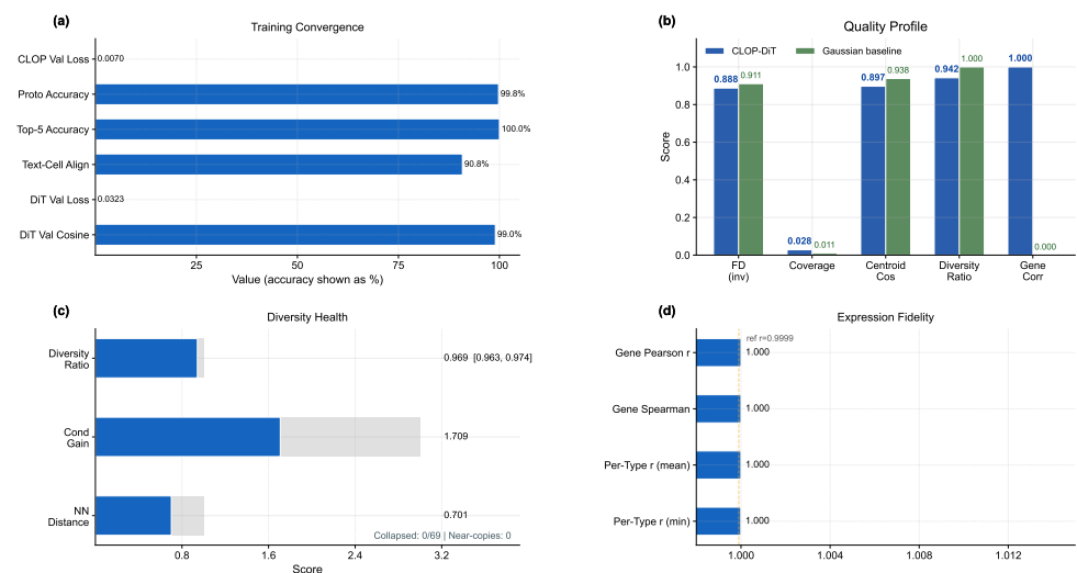
Figure 5. Metrics dashboard summarizing conditional generation quality. (a) Training convergence: normalized endpoint scores for loss reduction and accuracy/correlation with exact final values beside each row. (b) Quality profile bar chart showing multi-metric comparison between CLOP-DiT and Gaussian baseline (FD inv , coverage, centroid cosine, diversity ratio, gene correlation). (c) Diversity health gauges. (d) Expression fidelity bar chart. KNN accuracy (well above chance), steering accuracy (81%), diversity ratio, linear classifier accuracy, and Fréchet distance are shown across configurations. The collapse of unconditional generation to random baselines validates that text conditioning drives all cell-type specificity.
