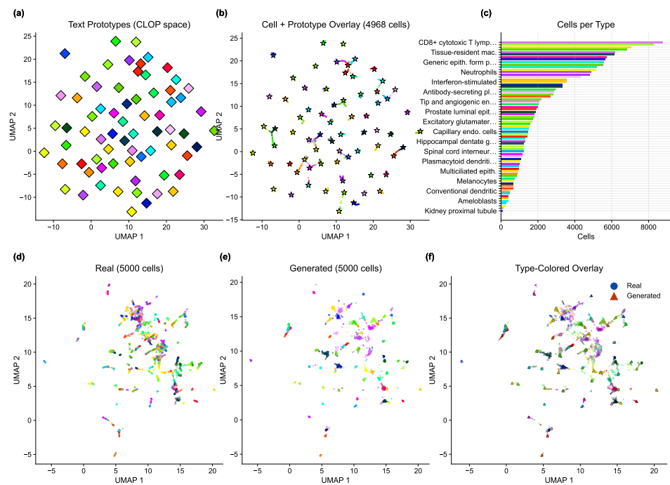
Figure 4. Embedding space analysis. (a) UMAP of text prototypes in the shared CLOP projection space, (b) cell embeddings with text prototype overlay (star markers) confirming co-localization of text and cell clusters (pairwise cosine = 0.222), and (c) cells-per-type bar chart with abbreviated type labels. (d) UMAP of real cells only (type-colored), (e) UMAP of generated cells only (type-colored), and (f) type-colored overlay of real (circles) and generated (triangles) cells. Generated cells occupy overlapping but distinguishable regions relative to their real counterparts.
