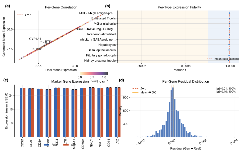
Figure 9. Expression correlation analysis. (a) Per-gene mean expression scatter (real vs. generated), with point color encoding absolute residual magnitude and outlier genes annotated. (b) Per-type Pearson r lollipop chart with threshold-band shading. (c) Marker gene expression (real vs. generated) grouped bars with error whiskers). (d) Per-gene residual distribution (generated – real) with percentage of genes within tolerance bands. High correlation confirms that the scGPT decoder faithfully reconstructs gene-level signatures from DiT-generated latent vectors. Caveat: because both real and generated profiles pass through the same frozen decoder, these high correlations measure decoder-reconstruction consistency, not generative fidelity (see Section 2.4).
