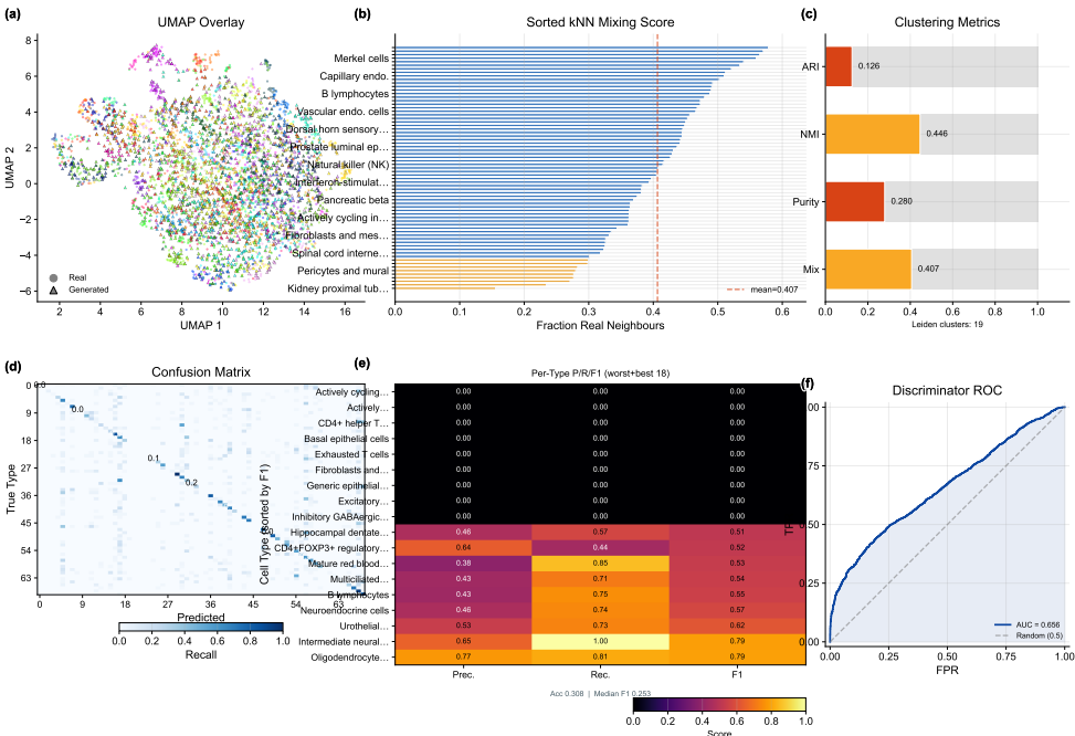
Figure 17. Downstream validation: clustering and classifier alignment. (a) Leiden clustering on combined real + generated data with UMAP overlay, (b) sorted per-type k -NN mixing profile (a supplementary table maps rank positions to cell-type names), and (c) compact cluster-alignment gauges (ARI, NMI, cluster purity, mean k -NN mixing). (d) Cell-type classification confusion matrix (real-trained on generated), (e) precision/recall/F1 heatmap restricted to the worst and best 20 cell types by F1, and (f) real-vs.-generated discriminator ROC curve. Median per-type F1 is reported in the heatmap stat box.
