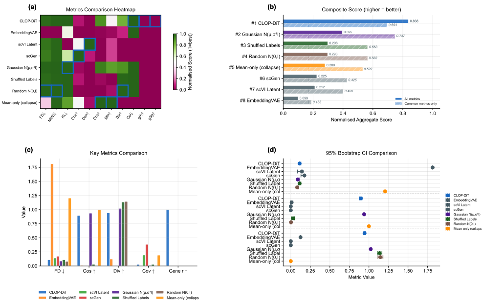
Figure 15. Composite benchmark across eight methods including scGen and scVI Latent external baselines. (a) Normalized metrics heatmap (methods \times metrics; green = high performance). (b) Composite score: solid bars show the full 17-metric composite, hatched bars show the common-metrics-only (9 shared distributional metrics) composite. (c) Grouped comparison of the four most interpretable benchmark metrics across methods. (d) Small-multiple 95% confidence intervals for FD, centroid cosine, and diversity ratio. On the full composite (0.838) CLOP-DiT ranks first, but on the common-metrics-only composite (0.694) it is outperformed by the Gaussian baseline (0.747), indicating that the overall advantage is driven by CLOP-DiT-exclusive downstream metrics. scGen achieves the highest coverage (0.384) among all methods.
