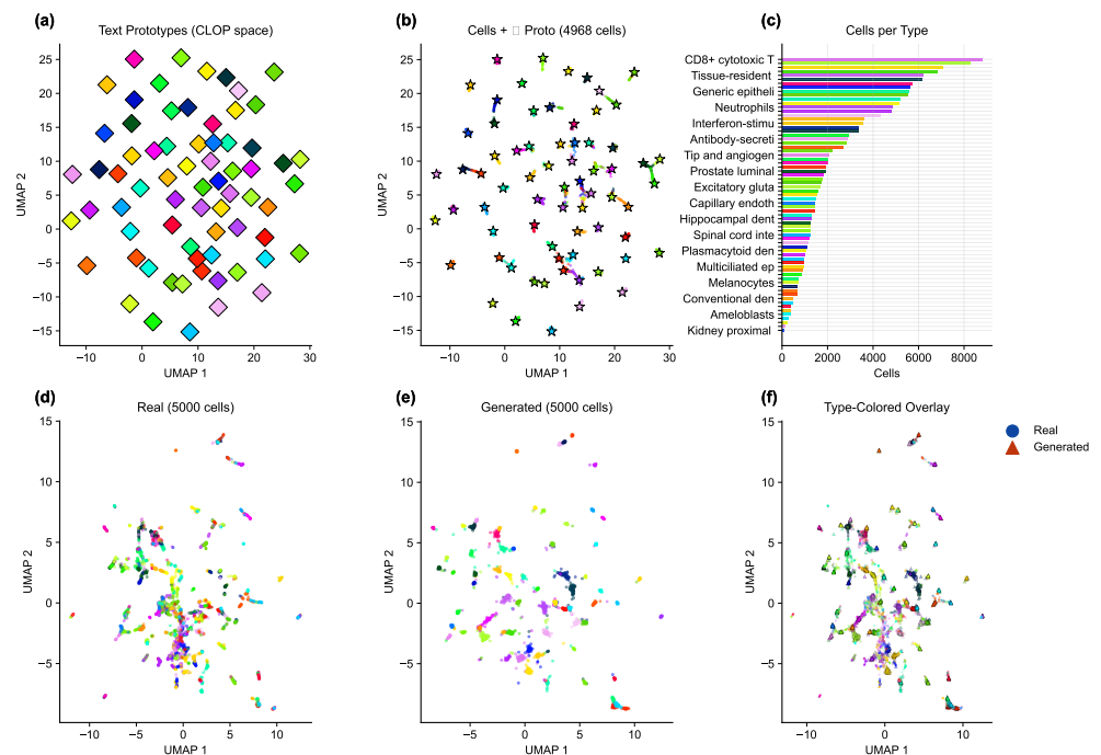
Figure 3. Embedding space analysis. (a) UMAP of text prototypes in the shared CLOP projection space, (b) cell embeddings with text prototype overlay (star markers) confirming co-localization of text and cell clusters (pairwise cosine = 0.222), and (c) cells-per-type bar chart with abbreviated type labels. (d) UMAP of real cells only (type-colored), (e) UMAP of generated cells only (type-colored), and (f) type-colored overlay of real (circles) and generated (triangles) cells. Generated cells occupy overlapping but distinguishable regions relative to their real counterparts.
