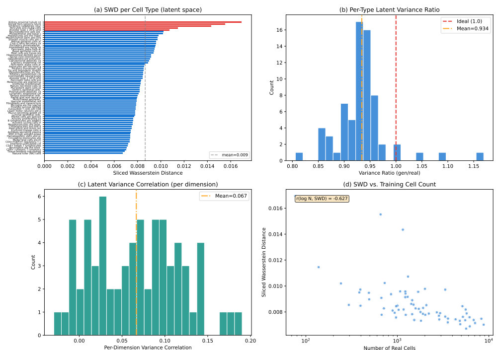
Figure 18. Pilot variance-matching analysis. (a) Per-cell-type sliced Wasserstein distance (SWD) between real and generated latent distributions, sorted by magnitude; red bars exceed one standard deviation above the mean. (b) Distribution of per-type latent variance ratios (gen/real); mean = 0.934, indicating that global variance magnitude is largely preserved. (c) Distribution of per-dimension variance correlations; mean = 0.067, confirming near-zero structural alignment despite preserved magnitude. (d) SWD vs. training cell count shows no strong correlation, suggesting that distributional mismatch is not simply a data-scarcity artifact.
