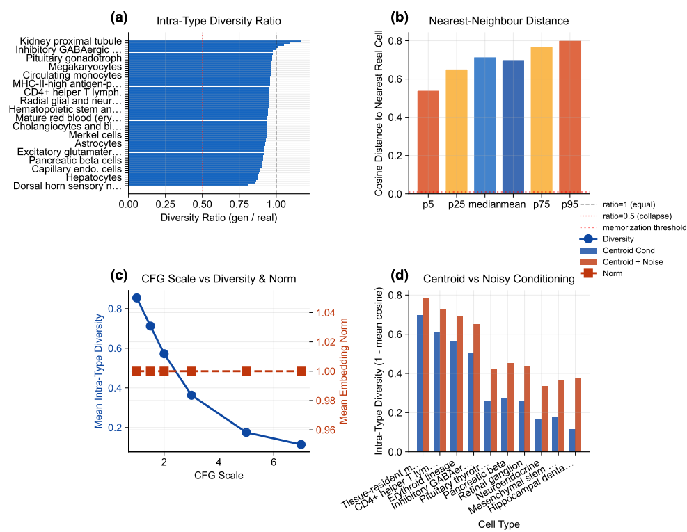
Figure 12. Diversity diagnostics. (a) Intra-type diversity ratio ranked across cell types (labels abbreviated for readability). (b) Nearest-neighbor distance distributions for real and generated populations. (c) CFG scale vs. diversity and norm trade-off across Euler and Midpoint solvers. (d) Centroid vs. noisy conditioning comparison. KNN accuracy saturates at CFG \approx 2.0–3.0 while diversity decreases monotonically.
