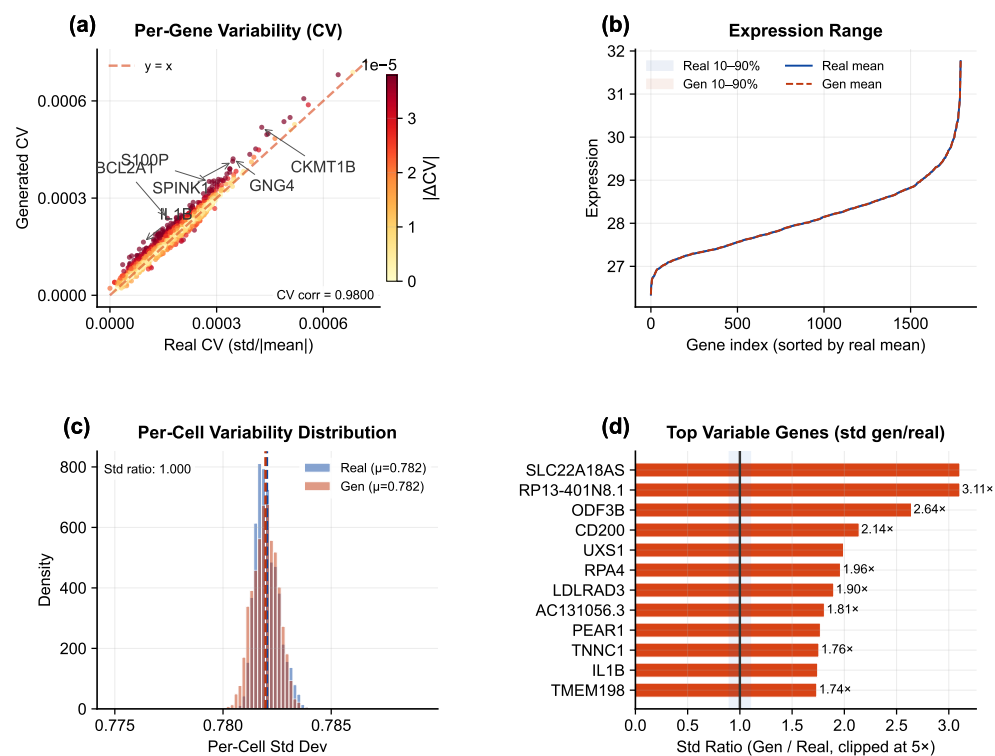
Figure 10. Expression distribution analysis. (a) Per-gene coefficient of variation scatter (real vs. generated) with outlier gene annotations. (b) Expression range ribbon with 10–90th and 25–75th percentile bands for real and generated cells. (c) Per-cell variability (standard deviation) distribution comparing real and generated populations. (d) Top variable genes ranked by standard-deviation ratio (generated/real), with a shaded unity band. Caveat: all expression panels reflect decoder-reconstructed profiles; high correlations indicate decoder consistency, not intrinsic generative accuracy (see Section 2.4).
