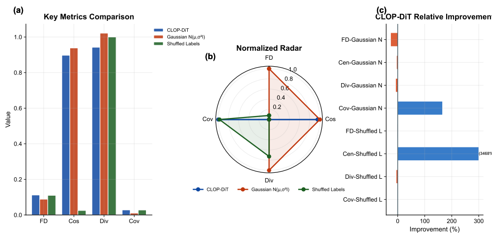
Figure 15. Baseline comparison. (a) Head-to-head grouped-bar analysis of CLOP-DiT vs. baselines (unconditional CFG = 0, Gaussian per-type sampling, decoder-only) across four evaluation metrics (Fréchet distance, centroid cosine similarity, diversity ratio, coverage). (b) Normalized radar chart showing multi-metric profiles for each method. (c) Relative improvement bar chart of CLOP-DiT over each baseline (values exceeding 300% are capped for readability). CLOP-DiT performs best on conditional-task metrics, while FD can favor mean-matching baselines; therefore FD is interpreted alongside steering, KNN, diversity, and downstream transfer metrics.
