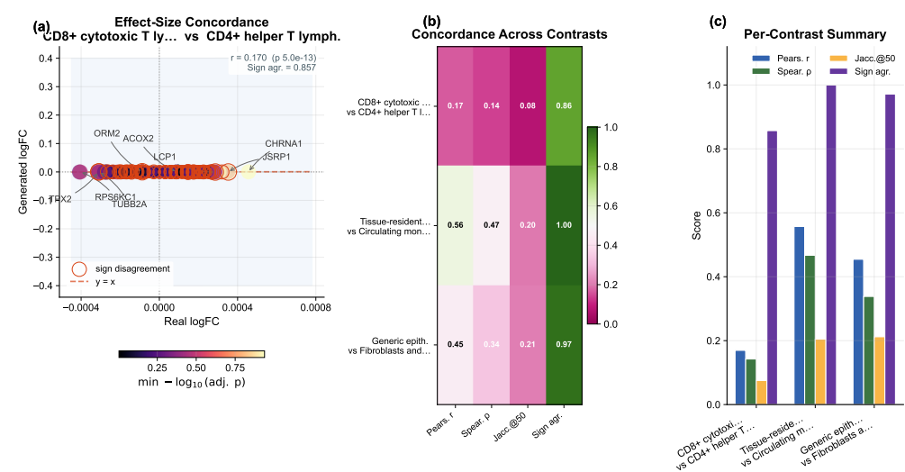
Figure 18. DE concordance. (a) Effect-size-weighted real-vs.-generated log-fold-change scatter for the leading contrast, with point size proportional to average absolute effect size and color indicating adjusted significance; sign-disagreement genes are outlined. (b) Compact summary heatmap reporting four metrics—Pearson r , Spearman \rho , Jaccard overlap of the top-50 DE genes (Jaccard@50), and sign agreement—across the three biologically meaningful contrasts (CD8 vs. CD4 T, resident macrophage vs. monocyte, epithelial vs. fibroblast). (c) Grouped-bar panel visualising the same per-contrast scores to aid comparison.
