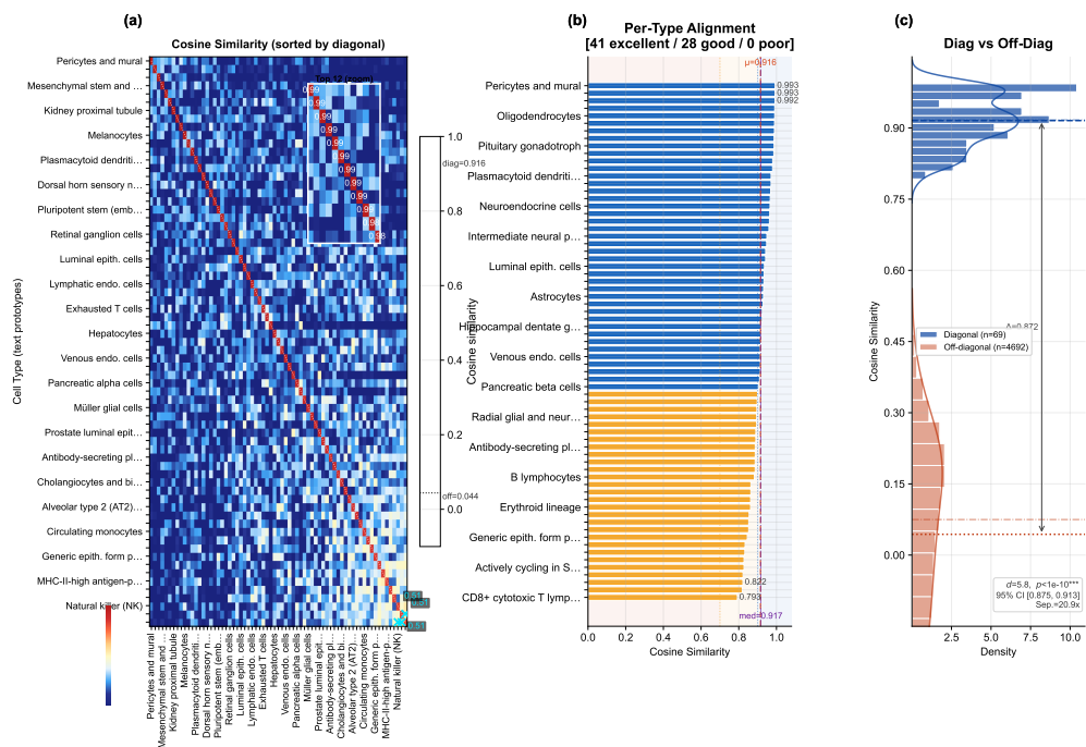
Figure 7. Text–cell alignment. (a) 69 \times 69 cosine similarity heatmap between text and cell centroids, sorted by diagonal similarity. Mean diagonal similarity \mu_{\text{diag}} = 0.916 ( \sigma = 0.053 ), mean off-diagonal \mu_{\text{off}} = 0.044 ( \sigma = 0.205 ); Cohen’s d = 5.8 , separation ratio 20.9\times , Mann–Whitney U p < 10^{-10} . (b) Per-type alignment bars color-coded by quality tier (41 excellent \geq 0.9 , 28 good, 0 poor). (c) Diagonal vs. off-diagonal distribution comparison with KDE overlay; the two populations are well separated ( \Delta = 0.872 , bootstrap 95% CI [0.875, 0.913]).
