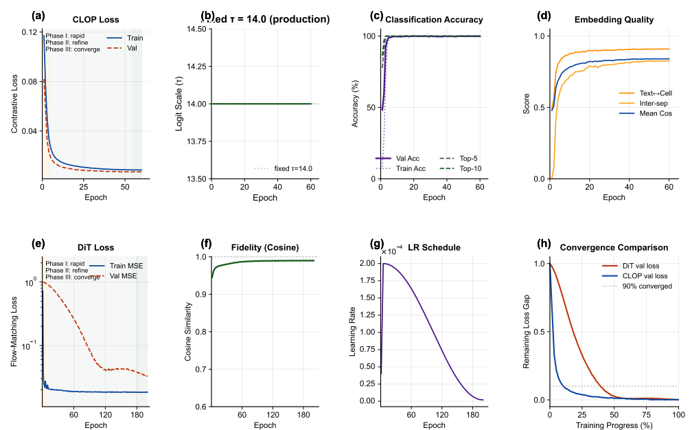
Figure 3. Training dynamics of the CLOP-DiT pipeline. (a) CLOP contrastive loss, (b) fixed logit-scale parameter ( \tau = 14.0 ; the production model uses a fixed value, though the v8.2 ablation baseline used a learnable \tau ; see Table 5), (c) batch classification accuracy, and (d) embedding quality metrics over 60 epochs. Despite modest validation accuracy ( \sim 2.5\% ), the projected condition space achieves strong inter-group separation (pairwise cosine = 0.222). (e) DiT train and validation MSE loss (log scale), (f) velocity cosine similarity, (g) learning rate schedule, and (h) normalized convergence comparison of CLOP and DiT validation losses, plotted against training progress (%); the dashed line marks the 90% convergence threshold. Final metrics: CLOP val loss = 8.5 \times 10^{-3} , prototype accuracy = 99.8%, 60 epochs; DiT val MSE = 3.2 \times 10^{-2} , val cosine = 0.990, final LR = 2.0 \times 10^{-6} , EMA decay = 0.9999, 10-step Euler sampler, 200 epochs.
