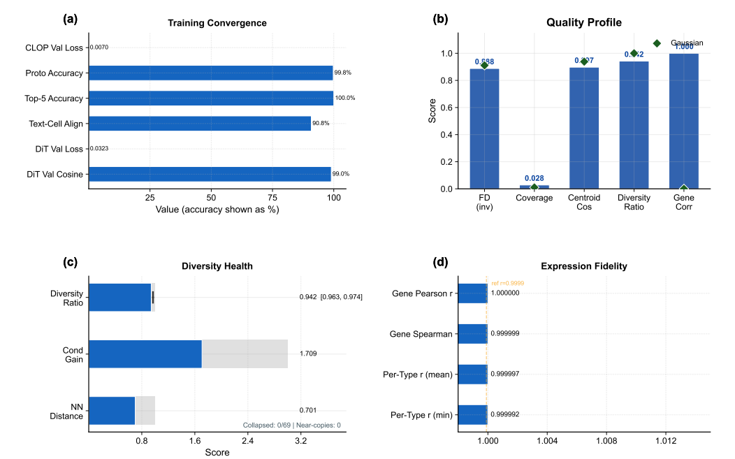
Figure 5. Metrics dashboard summarizing conditional generation quality. (a) Training convergence: normalized endpoint scores for loss reduction and accuracy/correlation with exact final values beside each row. (b) Quality profile bar chart showing multi-metric comparison between CLOP-DiT and Gaussian baseline (FD inv , coverage, centroid cosine, diversity ratio, gene correlation). (c) Diversity health gauges. (d) Expression fidelity bar chart. KNN accuracy (well above chance), steering accuracy (81%), diversity ratio, linear classifier accuracy, and Fréchet distance are shown across configurations. The collapse of unconditional generation to random baselines validates that text conditioning drives all cell-type specificity.
