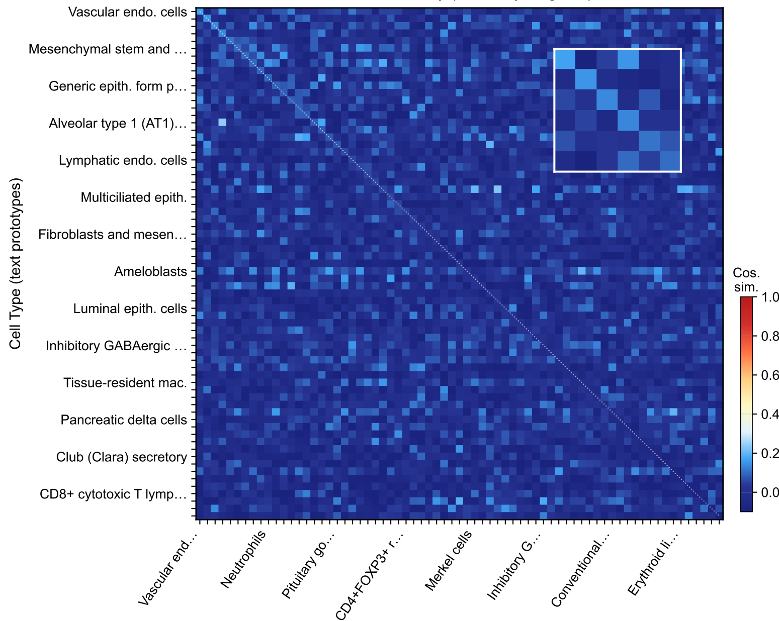
Cosine Similarity (sorted by diagonal)
