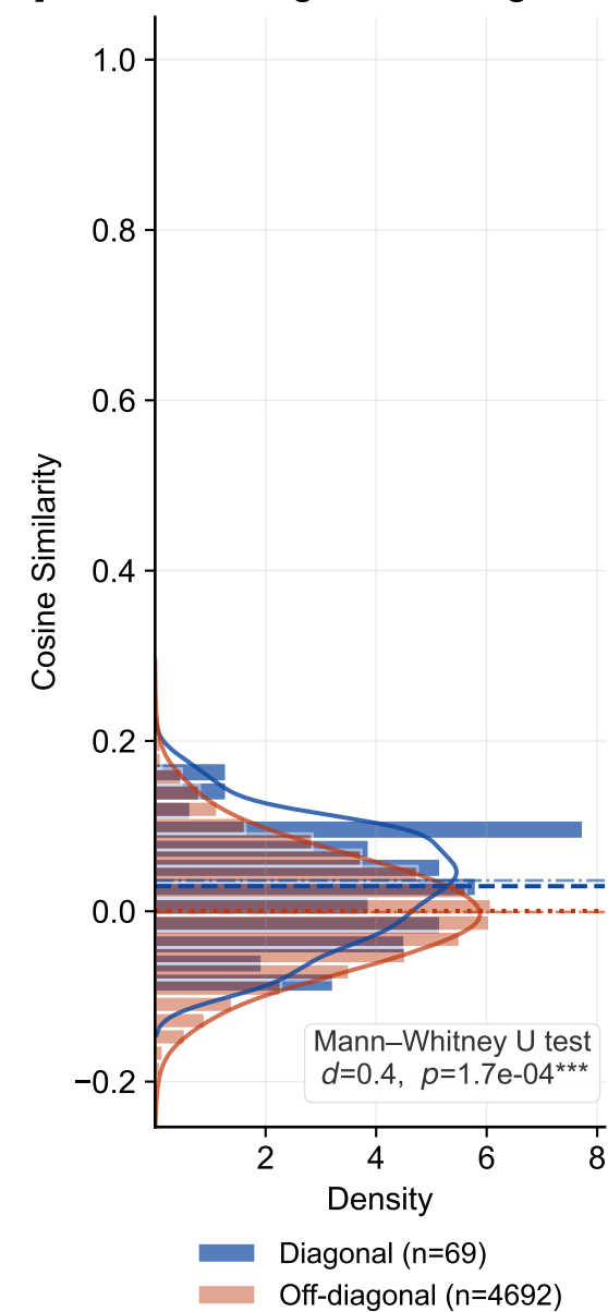
Diag vs Off-Diag
