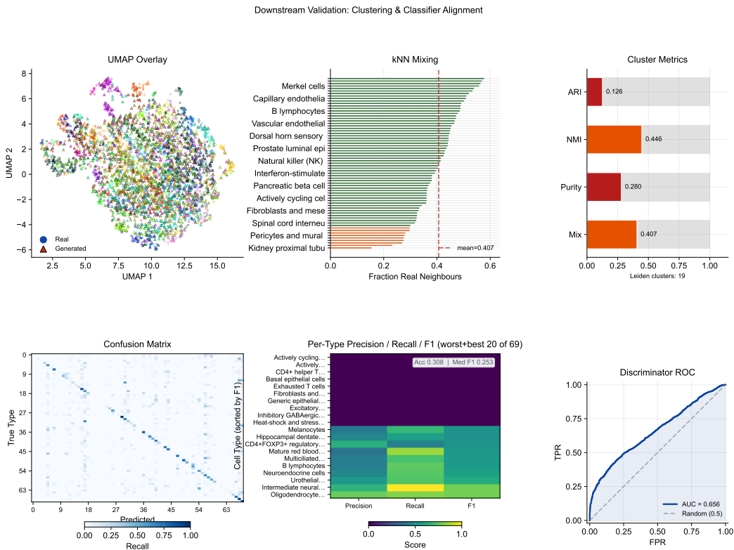
Figure 14. Downstream validation: clustering and classifier alignment. Top row: Leiden clustering on combined real + generated data with UMAP overlay, the lowest-mixing cell types, and compact cluster-alignment gauges (ARI, NMI, cluster purity, mean k -NN mixing). Bottom row: Cell-type classification confusion matrix (real-trained on generated), a precision/recall/F1 heatmap restricted to the worst and best 20 cell types by F1, and the real-vs.-generated discriminator ROC curve. This layout exposes which cell types are genuine downstream failures versus near-perfect transfers. Overall classifier accuracy on generated cells, macro F1, and discriminator AUC are reported in the main text (values from pipeline run).
