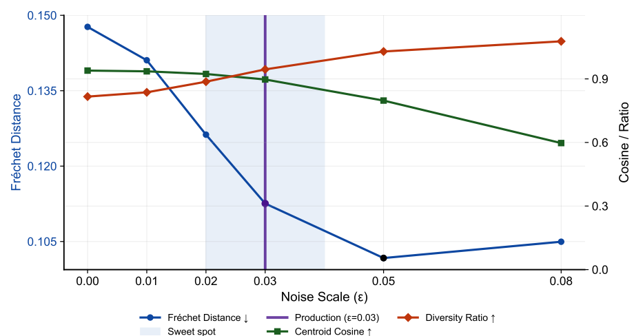
Figure 13. Noise-scale trade-off. (a) Fréchet distance (left axis), centroid cosine similarity, and diversity ratio (right axis) as a function of noise scale \epsilon at CFG = 1.5. The production configuration ( \epsilon = 0.03 ) is highlighted; a shaded band marks the sweet-spot region.
