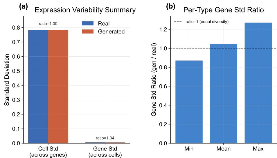
Figure 14. Expression-level diversity. (a) Gene-expression variability summary comparing real and generated populations across key statistics. (b) Per-type gene standard-deviation ratio (generated/real), confirming that the recommended Midpoint solver preserves biologically meaningful variance.
