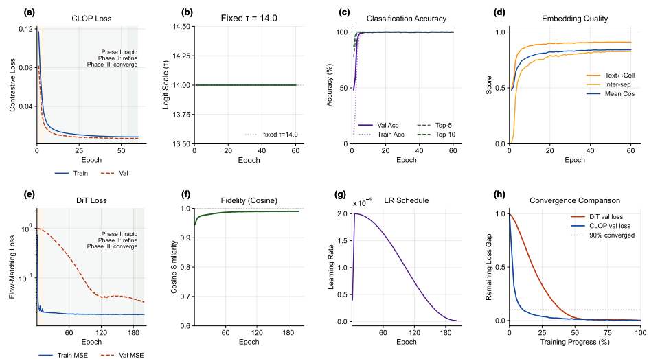
Figure 3. Training dynamics of the CLOP-DiT pipeline. (a–d) CLOP loss, fixed logit scale, batch accuracy, and embedding-quality metrics over 60 epochs. (e–h) DiT train/validation loss, velocity cosine similarity, learning-rate schedule, and normalized convergence comparison across training progress. Together, the panels show stable CLOP separation and near-converged DiT velocity prediction.
