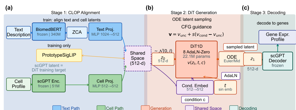
Figure 1. Overview of the CLOP-DiT pipeline. Stage 1 (CLOP) aligns structured text descriptions and scGPT cell embeddings in a shared 512-dimensional space after BiomedBERT whitening and projection. Stage 2 (DiT) performs conditional flow matching in scGPT latent space and generates a target latent from Gaussian noise using classifier-free guidance at inference. Stage 3 (Decoding) maps the generated latent back to gene expression through the frozen scGPT decoder.
