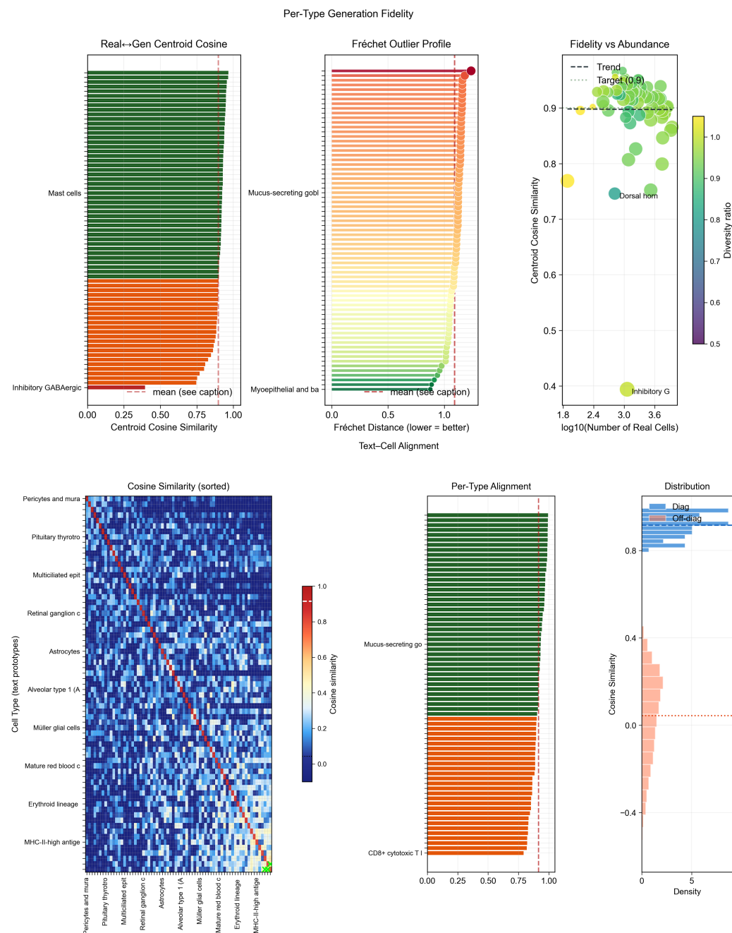
Figure 5. Per-type fidelity and text-cell alignment. Top row: Per-type centroid cosine similarity ranked across cell types, a Fréchet outlier profile with the global mean marked, and an abundance–fidelity scatter in which bubble size is proportional to Fréchet distance and colour encodes the per-type diversity ratio. Specific outlier type names are omitted from the bar panels for readability and are described in the surrounding text rather than directly on the bars. Together these panels expose the heterogeneity of generation quality across cell types instead of collapsing it to one mean score. Bottom row: 69×69 cosine similarity heatmap between text and cell centroids (strong diagonal dominance), per-type alignment bars, and diagonal vs. off-diagonal distribution comparison.
