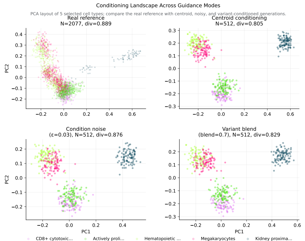
Figure 9. Conditioning landscape. Two-row PCA layout of the CLOP condition space showing the real reference cloud together with centroid, noisy, and variant-conditioned generations. Panel titles report the number of displayed cells and the mean within-type diversity for each conditioning mode, making the text-to-cell steering trade-offs easier to compare across modes.
