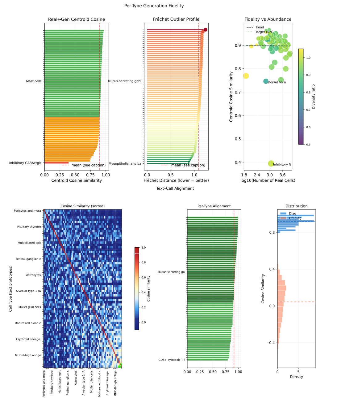
Figure 5. Per-type fidelity and text-cell alignment. Top row: Per-type centroid cosine similarity ranked across cell types, a Fréchet outlier profile with the global mean marked, and an abundance-fidelity scatter in which bubble size is proportional to Fréchet distance and colour encodes the per-type diversity ratio. Specific outlier type names are omitted from the bar panels for readability and are described in the surrounding text rather than directly on the bars. Together these panels expose the heterogeneity of generation quality across cell types instead of collapsing it to one mean score. Bottom row: 69×69 cosine similarity heatmap between text and cell centroids (strong diagonal dominance), per-type alignment bars, and diagonal vs. off-diagonal distribution comparison.
