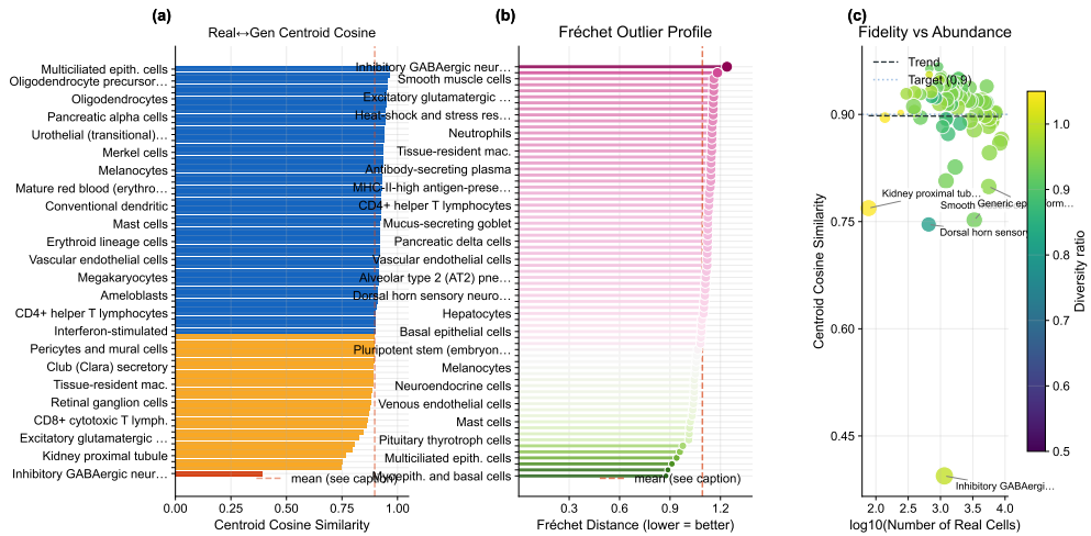
Figure 6. Per-type generation fidelity. (a) Per-type centroid cosine similarity ranked across cell types, (b) Fréchet outlier profile with the global mean marked, and (c) abundance–fidelity scatter (bubble size \propto Fréchet distance, color encodes diversity ratio). Cell-type names are mapped by rank position in the supplementary materials.
