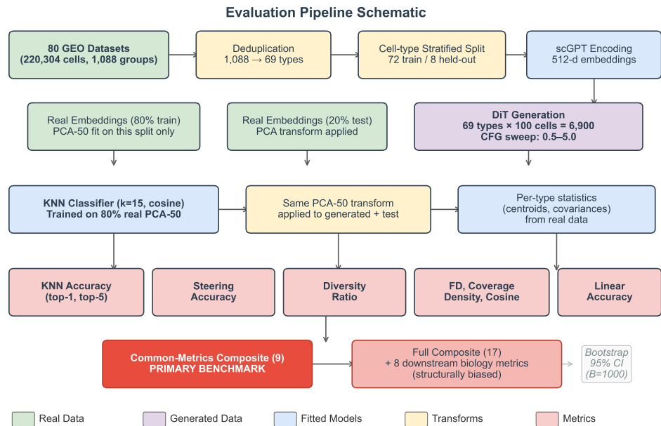
Figure 2. Evaluation pipeline schematic. Data flow from raw datasets through deduplication, stratified splitting, scGPT encoding, PCA fitting (on real training split only), KNN classifier training, and metric computation. The common-metrics-only composite (9 shared distributional metrics, marked in red) is the primary benchmark; the full 17-metric composite includes 8 downstream biology metrics reported only by CLOP-DiT and is structurally biased. Bootstrap confidence intervals ( B=1,000 ) are computed by resampling the 69 evaluation types.
