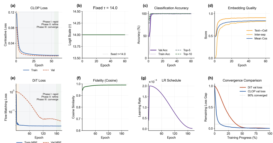
Figure 3. Training dynamics of the CLOP-DiT pipeline. (a–d) CLOP loss, fixed logit scale, batch accuracy, and embedding-quality metrics over 60 epochs. (e–h) DiT train/validation loss, velocity cosine similarity, learning-rate schedule, and normalized convergence comparison across training progress. Together, the panels show stable CLOP separation and near-converged DiT velocity prediction.
