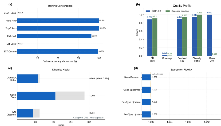
Figure 5. Metrics dashboard summarizing conditional generation quality. (a) Training convergence summary. (b) Multi-metric comparison between CLOP-DiT and the Gaussian baseline, including inverse FD, coverage, centroid cosine, diversity ratio, and per-gene Pearson correlation. (c) Diversity health gauges. (d) Expression-fidelity summary across configurations.
