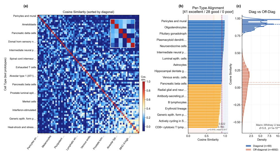
Figure 7. Text–cell alignment. (a) 69 \times 69 cosine similarity heatmap between text and cell centroids, sorted by diagonal similarity. Mean diagonal similarity \mu_{\text{diag}} = 0.916 ( \sigma = 0.053 ), mean off-diagonal \mu_{\text{off}} = 0.044 ( \sigma = 0.205 ); Cohen's d = 5.8 , separation ratio 20.9\times , Mann–Whitney U p < 10^{-10} . (b) Per-type alignment bars color-coded by quality tier (41 excellent \geq 0.9 , 28 good, 0 poor). (c) Diagonal vs. off-diagonal distribution comparison with KDE overlay; the two populations are well separated ( \Delta = 0.872 , bootstrap 95% CI [0.875, 0.913]).
