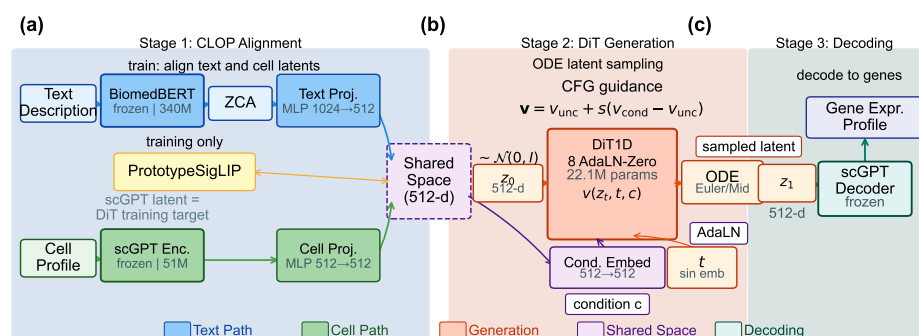
Figure 1. Overview of the CLOP-DiT pipeline. Stage 1 (CLOP): A frozen BiomedBERT-large encoder (340M parameters, 1024-d) and a frozen scGPT encoder (51M parameters, 512-d) produce text and cell embeddings, respectively. Dual MLP projectors map both modalities to a shared 512-dimensional L_2 -normalized space, trained with a PrototypeSigLIP contrastive loss. ZCA whitening is applied to BiomedBERT embeddings prior to projection. Stage 2 (DiT): A 1D Diffusion Transformer (8 AdaLN-Zero blocks, 22.1M parameters) performs conditional flow matching in the 512-dimensional scGPT latent space, using CLOP-projected text as the conditioning signal. An Euler or Midpoint ODE solver integrates the learned velocity field from Gaussian noise z_0 \sim \mathcal{N}(0, I) to a generated latent z_1 . Classifier-free guidance (CFG) is applied at inference. Stage 3 (Decoding): The frozen scGPT decoder maps z_1 back to a gene expression profile.
