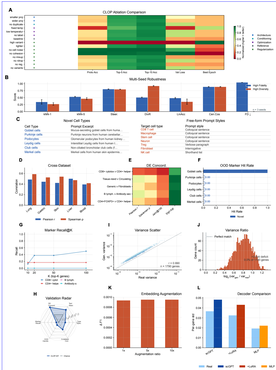
Figure A1: Supplementary validation, ablation, and expression fidelity. (a–e) A–C Robustness and ablation: (a) CLOP ablation heatmap showing normalised metrics across 15 configuration variants with component-category markers ablations, (b) multi-seed generation robustness across the high-fidelity and high-diversity operating regimes ( n = 3 independent seeds), and (c) out-of-distribution generation the OOD prompt showcase listing six novel cell types (unseen during training) and eight free-form natural-language prompts. (d–h) D–H Downstream validation suite: (d) cross-dataset mean-expression expression correlation (Pearson r and Spearman \rho ) across five held-out tissues, (e) expanded differential-expression concordance heatmap across five cell-type contrasts, (f) OOD marker-hit rates for novel cell types marker hits, (g) marker recall@K curves for six representative cell types, and (h) the six-axis validation radar summarising type specificity, text steering, DE concordance, marker recall, OOD handling, and cross-dataset correlation. (i–l) I–L Expression fidelity and decoder analysis: (i) per-gene variance scatter (log-log scale) between real and generated profiles, (j) variance-ratio distribution highlighting the fraction of genes with >2 -fold deficit, (k) embedding-level augmentation \Delta F1 at 1 \times , 5 \times , and 10 \times ratios, and (l) decoder ablation comparing frozen scGPT, LoRA-adapted scGPT, and a trained /LoRA/MLP decoder comparison.
