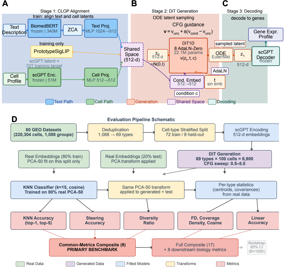
Figure 1: CLOP-DiT pipeline overview and evaluation framework. (Top) Stage-1 (CLOP) A–C : Stage 1 (CLOP) aligns structured text descriptions and scGPT cell embeddings in a shared 512-dimensional space after BiomedBERT whitening and projection. Stage-2 (DiT) : Stage 2 (DiT) performs conditional flow matching in scGPT latent space and generates samples a target latent from Gaussian noise using with classifier-free guidance at inference. Stage-3 (Decoding) : Stage 3 (Decoding) maps the generated sampled latent back to gene expression through the frozen scGPT decoder. (Bottom) Evaluation-D : evaluation pipeline schematic: data flow from raw datasets through deduplication, stratified splitting, scGPT encoding, PCA fitting (on real training the real-training split only), KNN classifier training, and metric computation. The common-metrics-only composite (9 shared distributional metrics) is the primary benchmark; bootstrap confidence intervals ( B=1,000 ) are computed by resampling the 69 evaluation types.
