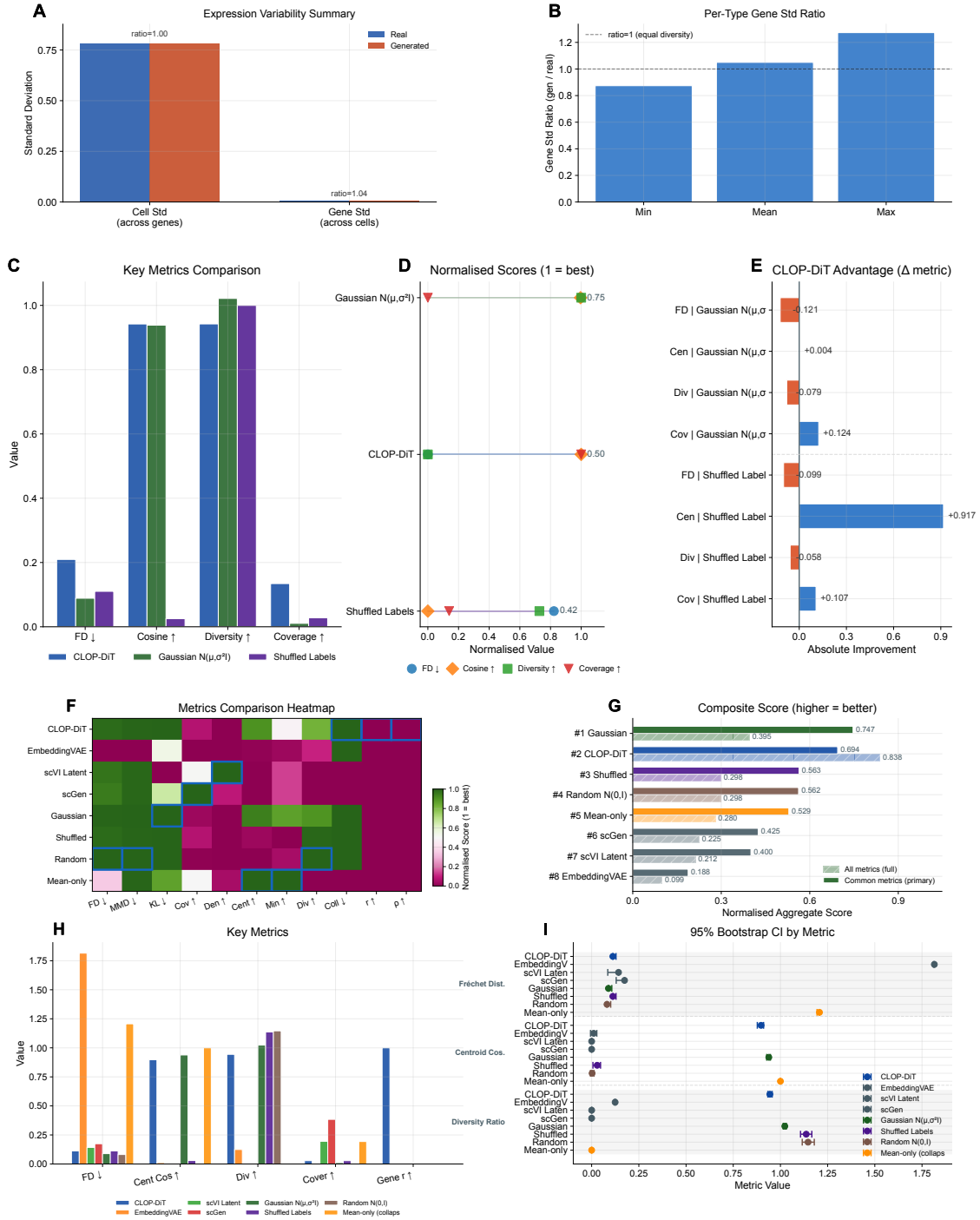
Figure 7: Expression-level diversity, baseline comparison, and composite benchmark. (Top) (a) A Gene-expression variability summary (real vs. generated). (b) B Per-type gene standard-deviation ratio. (Middle) (c) C Head-to-head grouped-bar analysis across four evaluation metrics. (d) D Ranked normalised scores per method. (e) E Absolute metric delta of CLOP-DiT relative to each baseline. (Bottom) (f) F Normalized metrics heatmap (methods \times metrics). (g) G Composite score (solid = common-metrics-only; hatched = full). Warning: the full composite is structurally biased ; the common-metrics-only bars are the fair comparison. (h) H Grouped comparison of four interpretable metrics. (i) I 95% bootstrap confidence intervals.
