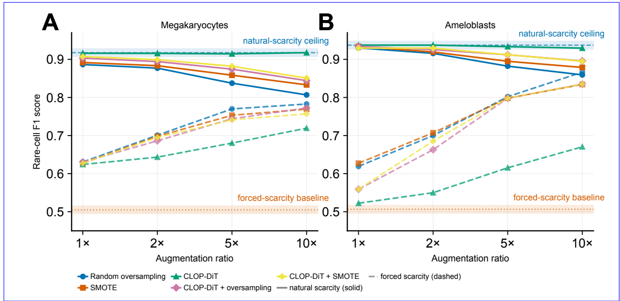
Figure A5: Forced-scarcity rescue: augmentation works when there is real headroom. Rare-class F1 as a function of augmentation ratio (1×, 2×, 5×, 10×) for two cell types — A Megakaryocytes, B Ameloblasts — under two scarcity regimes: natural scarcity (solid lines, baseline F1 > 0.92) and forced scarcity with 30 training cells per class (dashed lines, baseline F1 ≈ 0.50). Five strategies compared: random oversampling, SMOTE, CLOP-DiT-only, CLOP-DiT + oversampling, CLOP-DiT + SMOTE. Augmentation is flat or mildly negative under natural scarcity (ceiling-driven null) but recovers F1 by 0.2–0.35 under forced scarcity. The natural-scarcity null is therefore a ceiling artefact rather than a principled augmentation failure.
