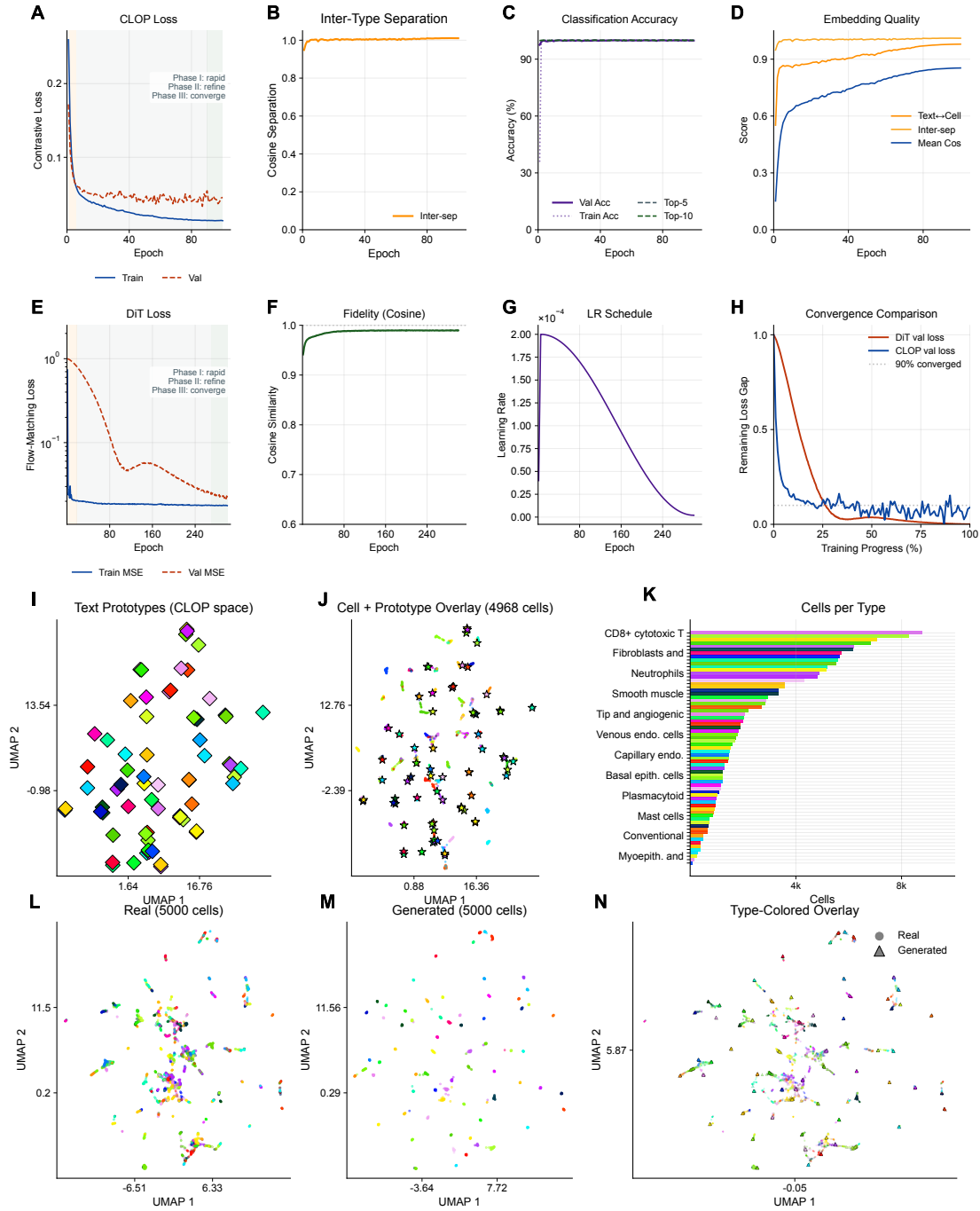
Figure 2: Training dynamics and embedding space analysis. Training dynamics (a-d) A-D CLOP loss, inter-type cosine separation, batch accuracy (shown on the full 0-100% scale to expose ceiling-like saturation of this stage-specific retrieval proxy), and embedding-quality metrics over the reported training run. (e-h) E-H DiT train/validation loss, velocity cosine similarity, learning-rate schedule, and normalized convergence comparison. Embedding space (i-j) I-J CLOP-projected text and cell embeddings form aligned clusters in the shared space. (k) K Cell-count distribution across types. (l-n) L-N Real and generated scGPT embeddings occupy overlapping but distinguishable regions.
