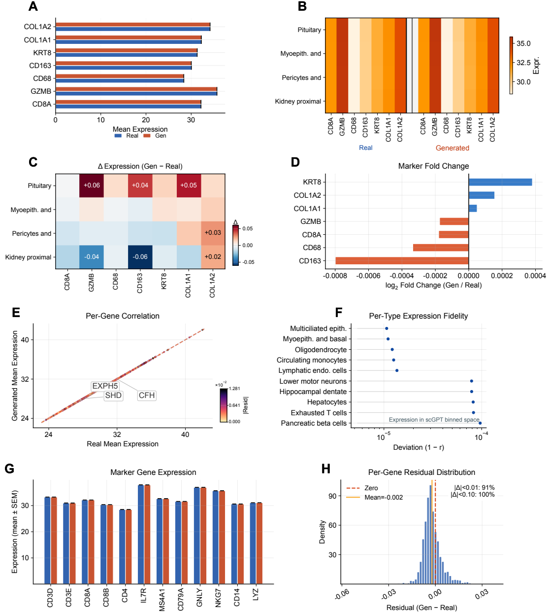
Figure 4: Gene-level fidelity analysis. Top-row (marker-gene-comparison): (a) Paired bar chart of canonical marker-gene expression in real vs. generated cells. (b) Per-type \times marker dual heatmap. (c) Difference heatmap ( \Delta = generated - real). Fold-change-waterfall (d) \log_2 fold-change summary across the marker panel. Bottom-row (expression-correlation): (e) Per-gene mean-expression scatter with residual coloring and short callouts for the largest outliers. (f) Per-type deviation from perfect correlation ( 1 - r , log scale). (g) Marker-gene expression comparison with error whiskers. (h) Per-gene residual distribution.
