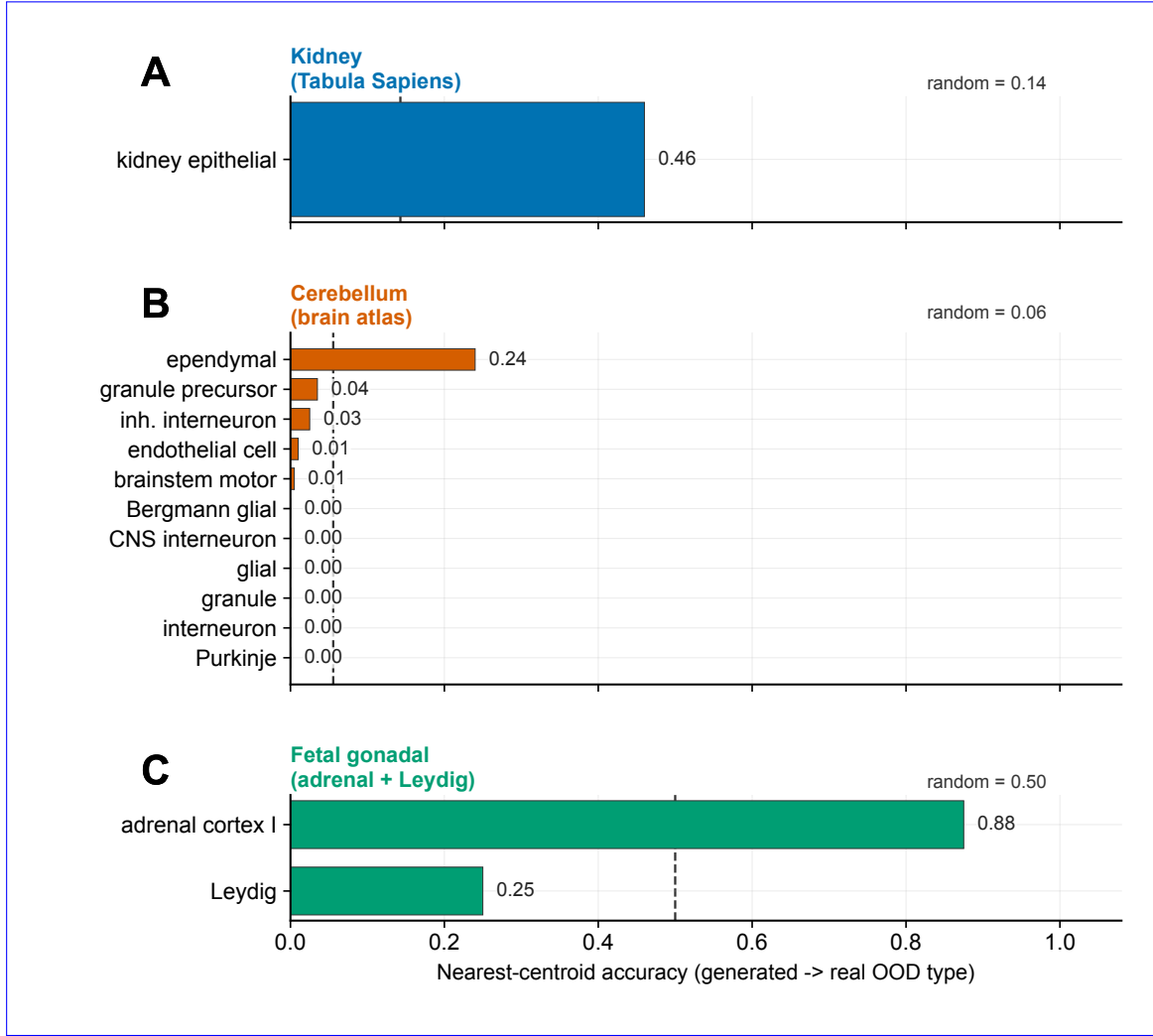
Figure 9: Zero-shot strict-ODD generalization of CLOP-DiT by novel cell type. Per-cell-type nearest-centroid accuracy for 14 cell types drawn from three strict-ODD tissues absent from the training corpus. Dashed lines mark random chance for the full OOD tissue vocabulary used by nearest-centroid scoring (1/7 kidney, 1/18 cerebellum, 1/2 fetal gonadal). Transfer is program-dependent: kidney epithelial reaches 0.460 on the 7-way kidney baseline, and adrenal cortex type I reaches 0.875 on the 2-way fetal-gonadal baseline, consistent with epithelial/steroidogenic overlap with training tissues. Structurally distinct cerebellar neural programs remain at or below chance because the training corpus has no neural analog. A further sibling-collapse failure mode appears on the fetal gonadal sample, where Leydig-prompted outputs concentrate near the dominant adrenal centroid.
