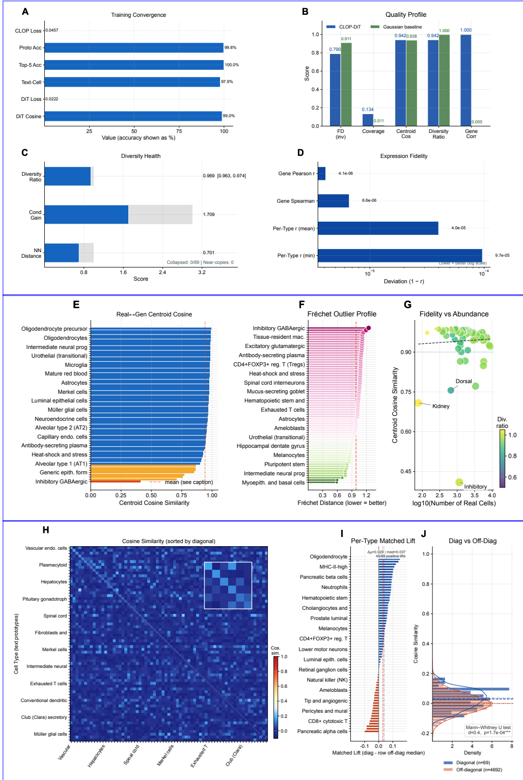
Figure 3: Generation quality overview: metrics, per-type fidelity, and text-cell alignment. Metrics dashboard (a) A Training convergence summary. (b) B Multi-metric comparison between CLOP-DiT and the versus Gaussian baseline. (c) metrics. C Diversity diversity health gauges. (d), and D Expression-fidelity-expression-fidelity deviation ( 1 - r_1 - r , log scale). Per-type fidelity (e) E Per-type-centroid cosine similarity-ranked across cell types by type, (f) F Fréchet outlier profile, and (g) G abundance-fidelity scatter. Text-cell alignment (h) H 69×69 text-prototype×cell-centroid cosine similarity-heatmap in CLOP-projected 512-d space (mean diagonal \mu_{\text{diag}} = 0.916 , \sigma = 0.053 , \mu_{\text{diag}} = 0.029 ; Cohen's d = 5.8 , separation ratio 20.9 \times d = 0.45 ). (i) I Per-type alignment bars matched lift, defined as matched text-cell similarity minus the row-wise off-diagonal median. (j) J Diagonal vs. versus off-diagonal distribution-comparison distributions ( \Delta = 0.872 , \Delta = 0.029 , bootstrap 95% CI 0.875[0.013, 0.045] , 0.913 Mann-Whitney p = 1.7 \times 10^{-4} ).
