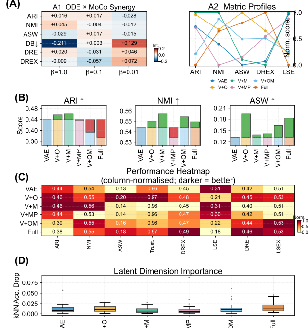
Fig. 3. Component contribution analysis (IRALL, \beta=0.1 ). (A) Two-part summary panel: A1 ODE \times MoCo interaction heatmap across metrics and \beta values, and A2 normalized metric profiles across configurations. (B) Incremental-gain waterfall for ARI, NMI, and ASW: each bar shows the marginal \Delta from the VAE baseline. (C) Column-normalised performance heatmap across eight metrics. (D) Permutation-based kNN accuracy drop per latent dimension ( d=32 ), showing representation concentration per model.
