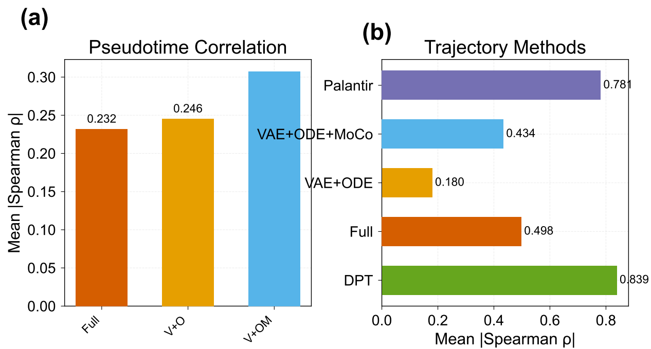
Fig. 14. Trajectory and pseudotime comparison. (a) Mean |Spearman \rho | between inferred pseudotime and collection day per ODE-containing configuration. (b) Trajectory baseline comparison: MoCoO vs. DPT and Palantir.
