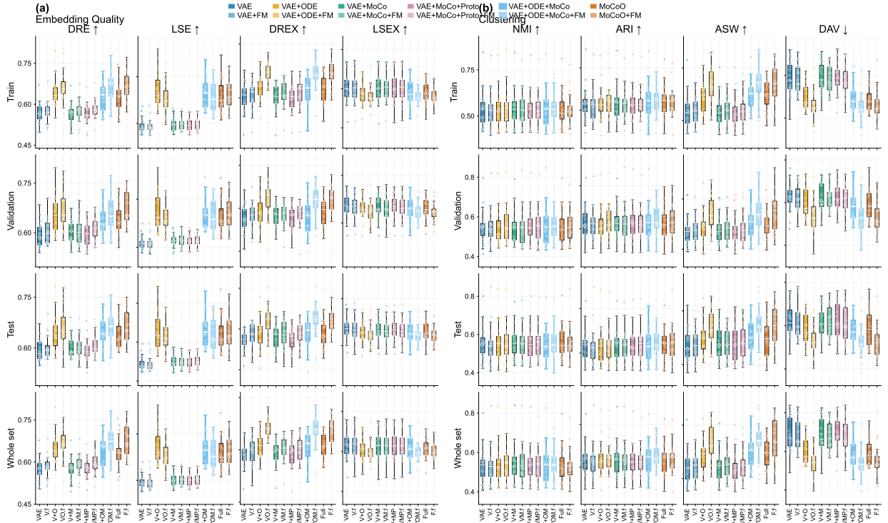
Fig. 4. Flow Matching enhancement across 20 datasets and 12 configurations (6 base + 6 FM-augmented). (a) Embedding quality metrics. (b) Clustering metrics. Thick-edged boxes with coloured borders highlight VAE+ODE+MoCo and VAE+ODE+MoCo+FM; the latter ranks top-two on six of eight metrics (Table VIII).
