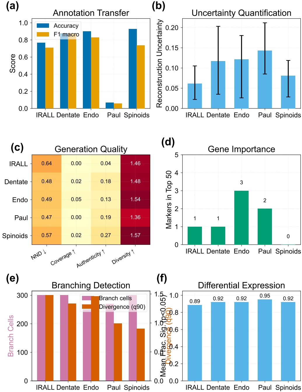
Fig. 5. Downstream biological validation across five datasets (Full MoCoO, \beta=0.1 ). (a) Annotation transfer: kNN accuracy and F1 macro per dataset. (b) Uncertainty quantification: mean uncertainty with 5th–95th percentile error bars. (c) Generation quality heatmap: nearest-neighbour divergence, coverage, authenticity, and diversity. (d) Gene importance: count of known lineage markers recovered in the top 50 latent-driving genes. (e) Branching detection: number of branch cells and q90 divergence per dataset. (f) Differential expression: mean fraction of significant genes ( p < 0.05 ) across clusters.
