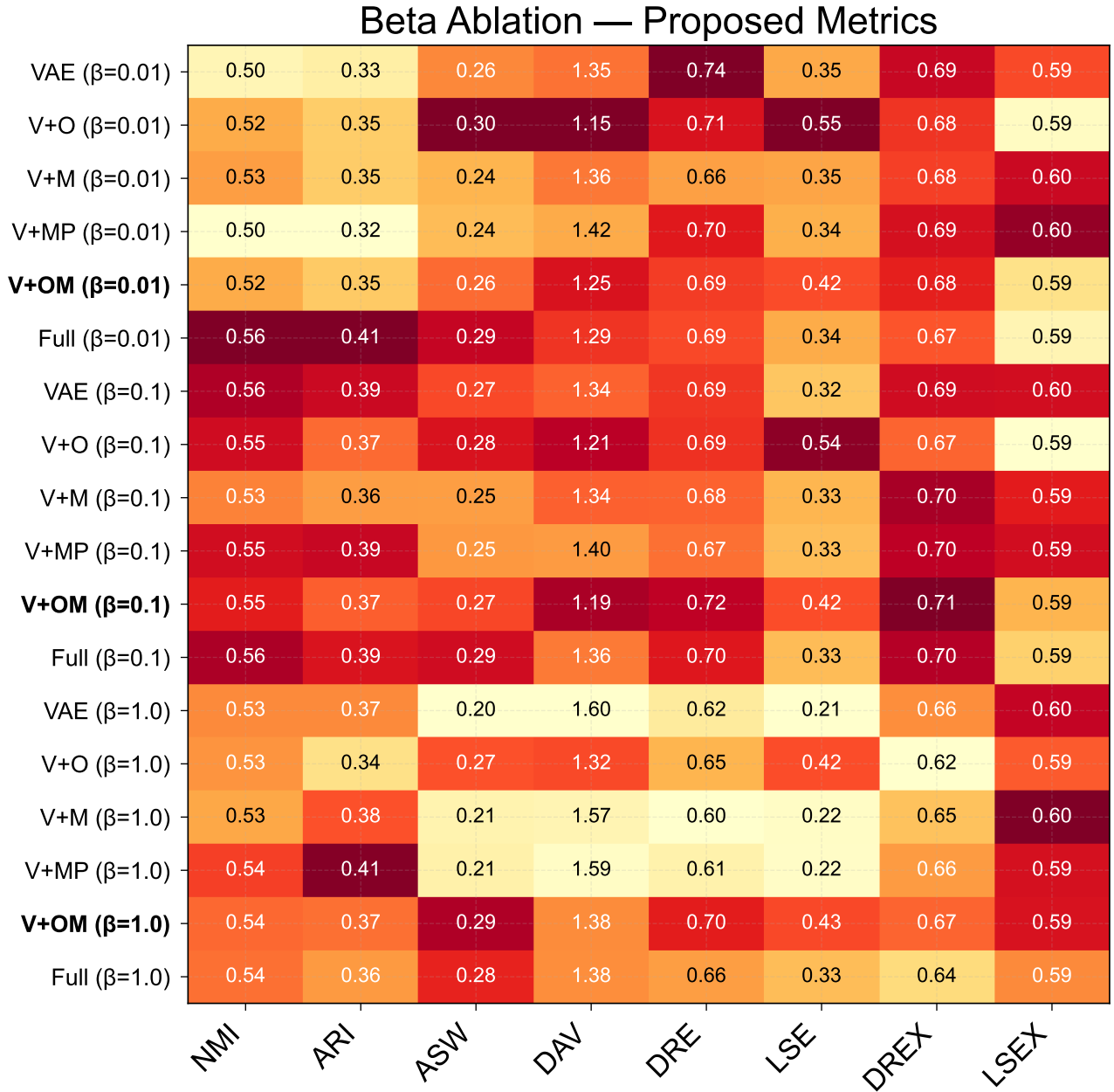
Fig. 15. Beta ablation heatmap. Each cell shows metric \times configuration at a given \beta value, with text annotations (.2f) and colour-mapped cells (column-normalised; higher = relatively better). Row labels for the VAE+ODE+MoCo configuration are emboldened for easy identification across all three beta settings.
