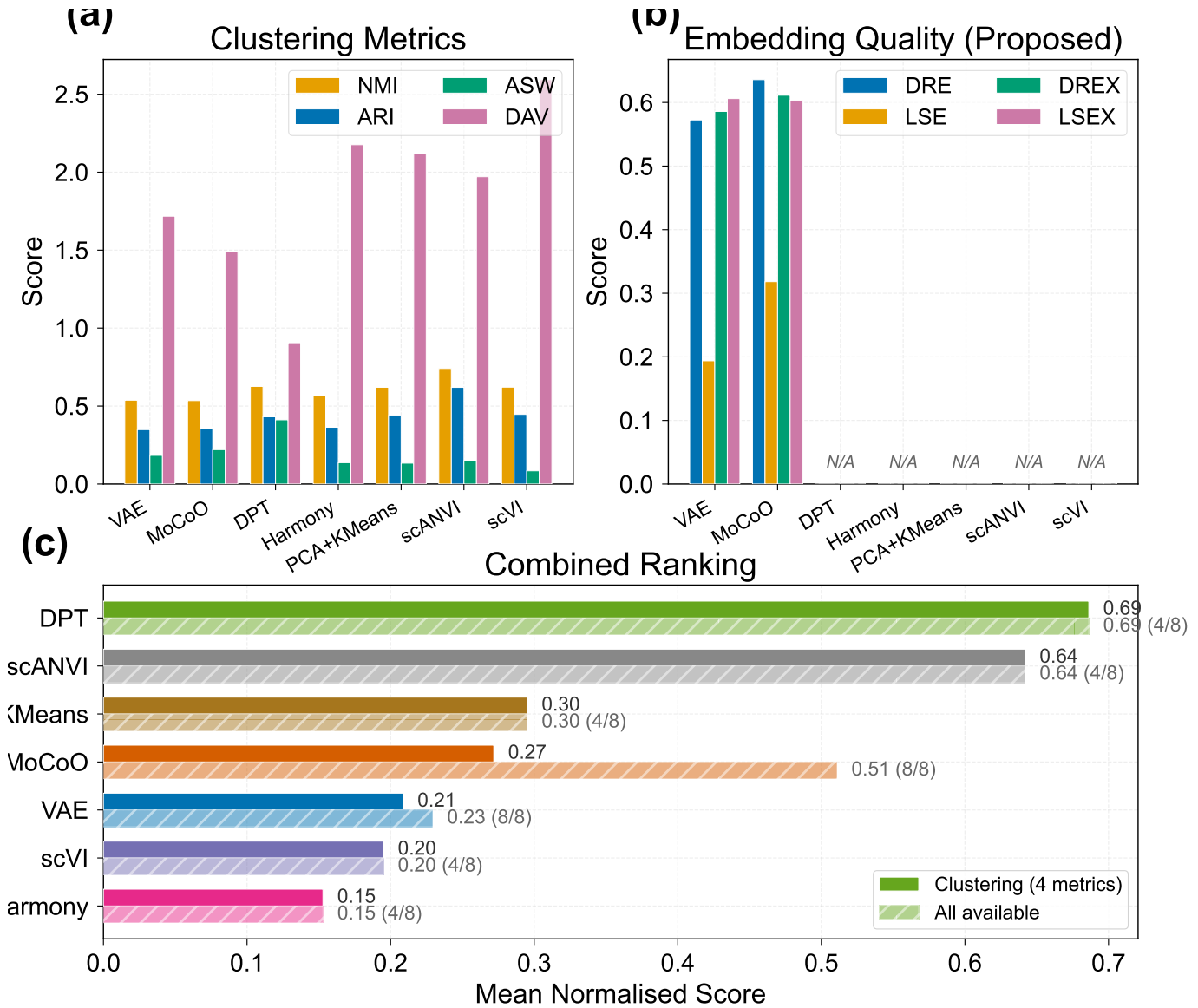
Fig. 13. External baseline comparison. (a) Clustering metrics (NMI, ARI, ASW, DAV) for MoCoO and external baselines. (b) Embedding quality metrics; hatched grey bars with “N/A” labels indicate metrics not computable for methods lacking a continuous latent representation. (c) Combined normalised ranking showing two bars per method: solid bars use only the 4 clustering metrics (available for all methods, providing a fair head-to-head comparison), while hatched bars average across all available metrics ( n/8 annotation). External methods’ two bars are identical because they only have clustering scores; MoCoO’s hatched bar additionally includes embedding quality. Sorted by clustering-only score to ensure like-for-like ordering.
