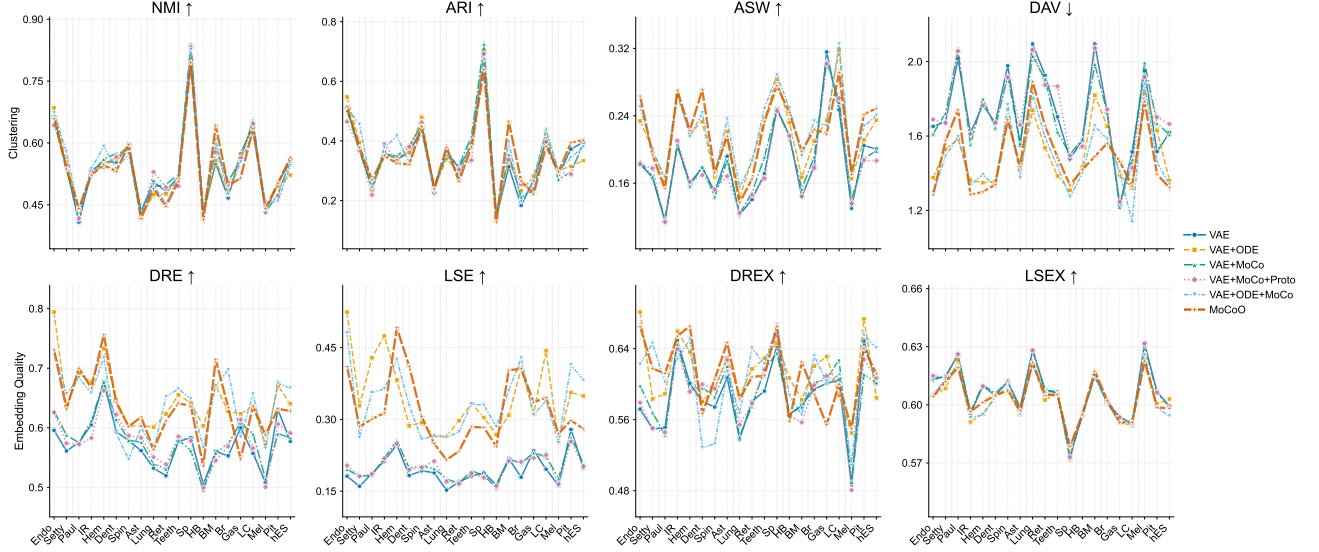
Fig. 3. Per-dataset metric profiles for each base configuration across 20 datasets. Line plots show metric variation (ARI, NMI, ASW, and embedding-quality metrics) across datasets, revealing dataset-specific strengths and cross-dataset consistency. ODE-containing configurations produce smoother developmental trajectories; VAE+ODE achieves the best overall embedding quality (Table IV).
