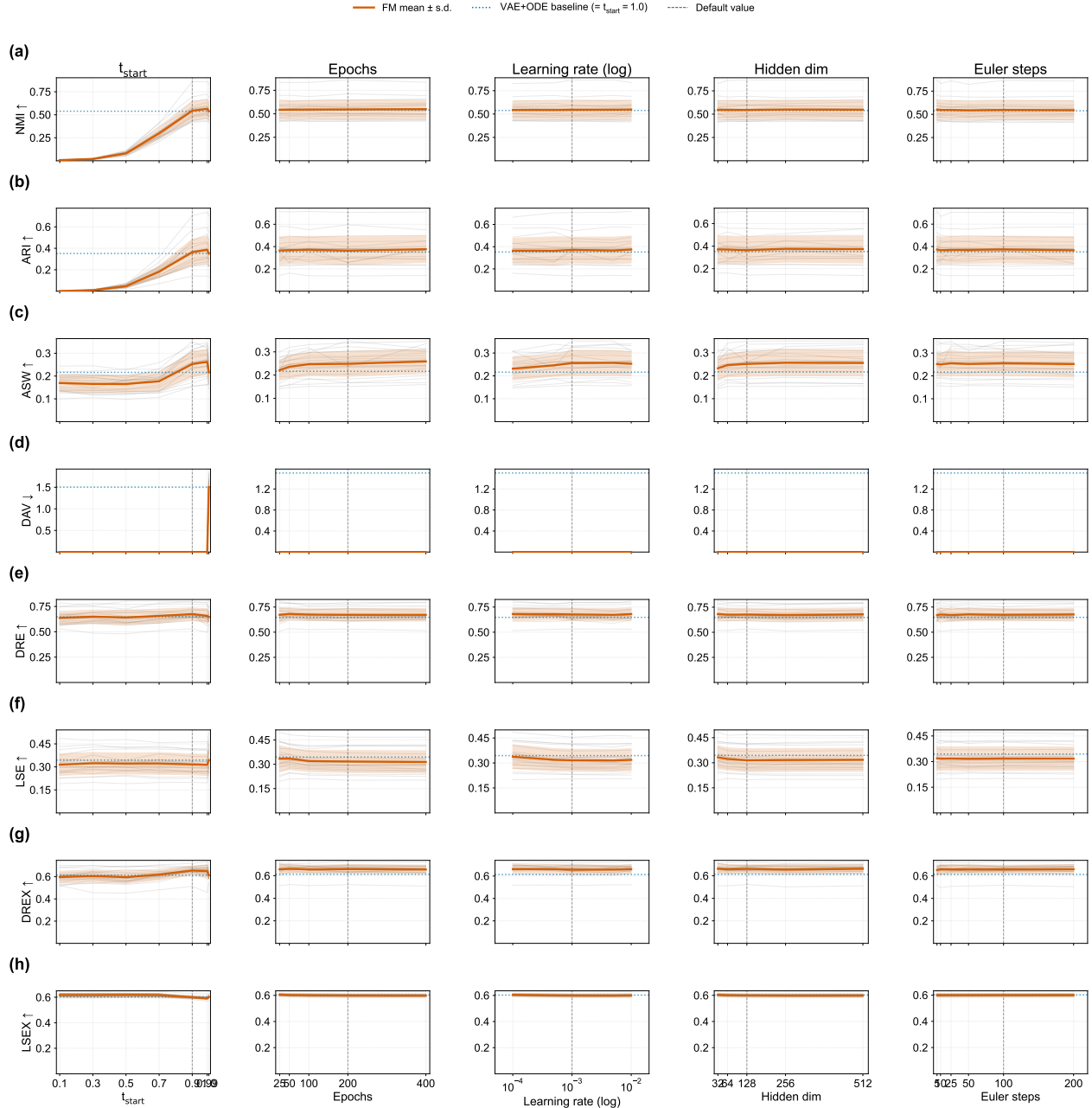
Fig. 6. FM hyperparameter sensitivity analysis across all datasets and the proposed 8-metric set (NMI, ARI, ASW, DAV, DRE, LSE, DREX, LSEX). Each row shows one metric; each column shows one hyperparameter. Per-dataset thin lines are overlaid with the mean (bold line) and \pm 1 s.d. shading. Vertical dashed lines mark default values; horizontal dotted lines show the VAE+ODE baseline (no FM).
