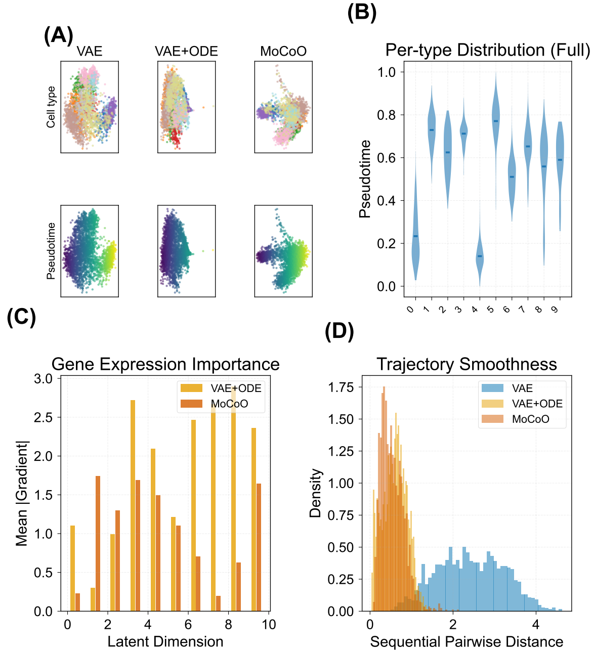
Fig. 9. ODE-driven pseudotime and trajectory analysis (IRALL). (A) PCA of latent spaces coloured by cell type (top row) and pseudotime (bottom row) for three representative configurations (VAE, VAE+ODE, Full); ODE adds temporal directionality. (B) Per-cell-type pseudotime distributions (violin plots, Full model); the ODE model separates developmental stages more continuously. (C) Per-dimension gradient magnitude across configurations, quantifying gene expression importance along the ODE axis. (D) Trajectory smoothness: sequential pairwise distance histograms per configuration.
