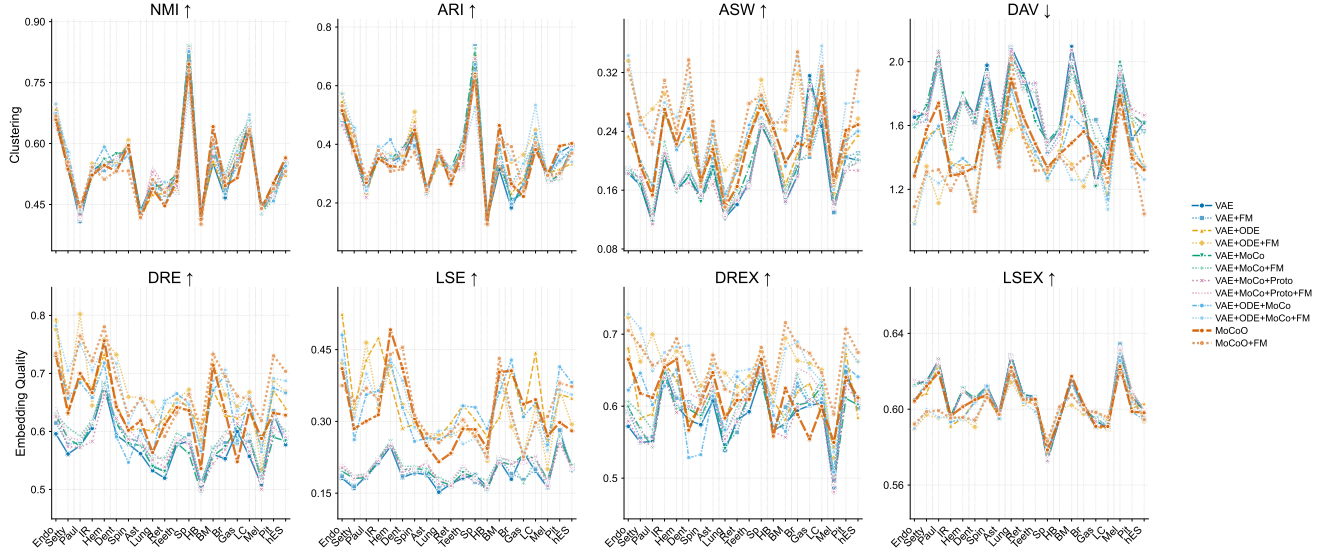
Fig. 7. FM-enhanced per-dataset metric profiles showing all 12 configurations (6 base + 6 FM variants). Each subplot shows one metric across datasets, with FM variants plotted alongside their base counterparts.
