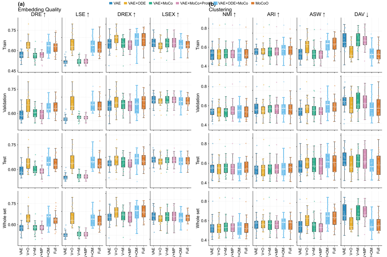
Fig. 2. Cross-dataset ablation across six MoCoO configurations and 20 scRNA-seq datasets. (a) Embedding quality metrics (DRE, LSE, DREX, LSEX). (b) Clustering metrics (ARI, NMI, ASW, DAV). Boxplots show the distribution across datasets per configuration; thick-edged boxes with coloured borders denote the VAE+ODE+MoCo configuration for easy identification.
