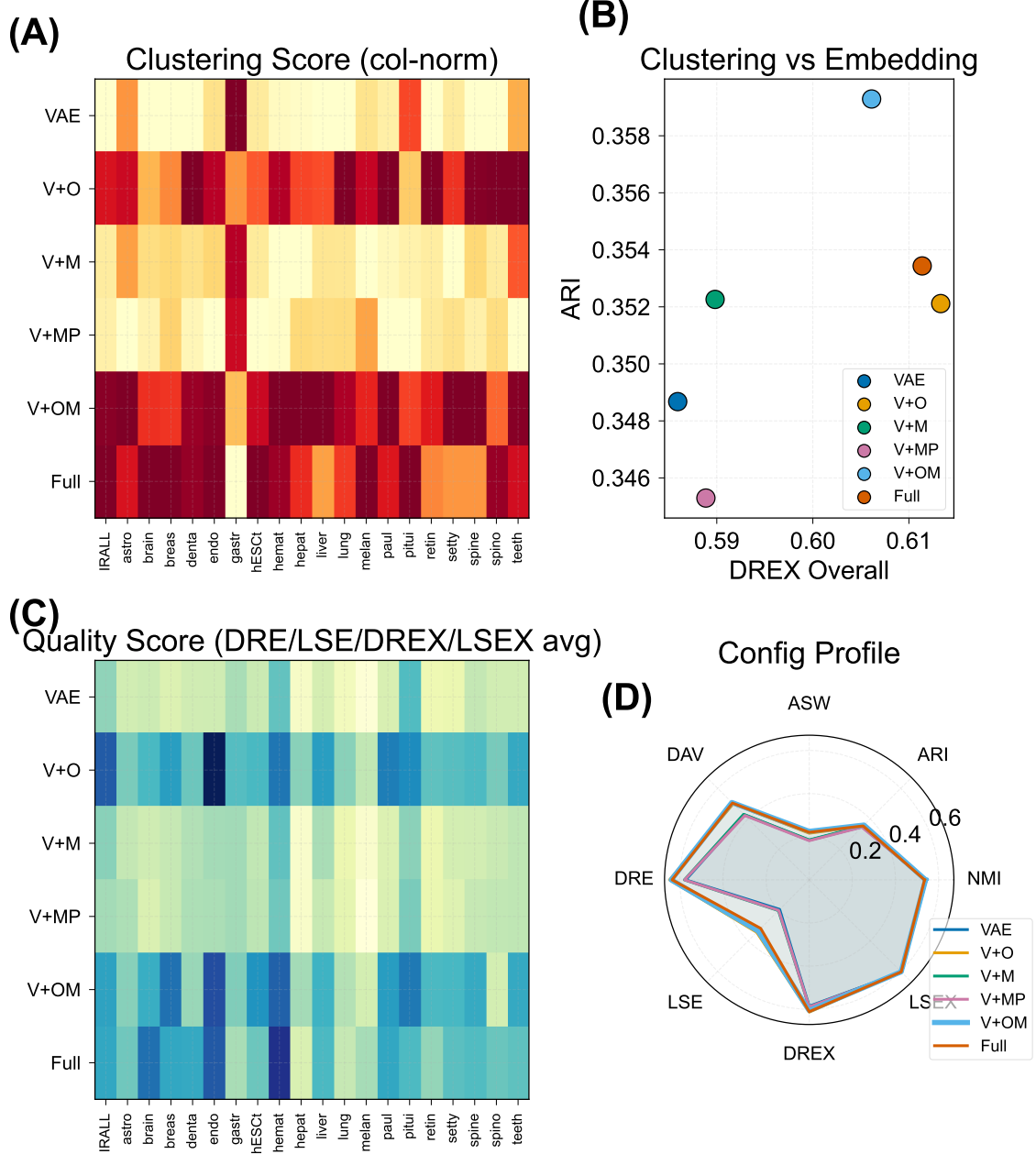
Fig. 10. Cross-dataset evaluation and generalization. (A) Column-normalised ARI heatmap (config \times dataset) across all 20 datasets. (B) ARI vs. DREX scatter (mean across datasets); VAE+ODE+MoCo achieves the strongest joint clustering–quality trade-off. (C) Average embedding quality (DRE, LSE, DREX, LSEX mean) heatmap across all 20 datasets. (D) Radar profile of all eight proposed metrics averaged across datasets; the VAE+ODE+MoCo polygon (thick border, filled) covers the largest area, confirming top-tier performance across metric families.
