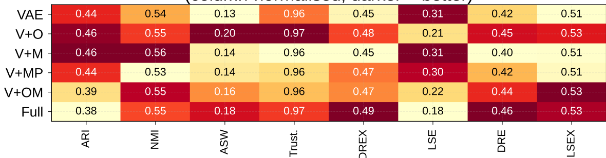
Performance Heatmap (column-normalised; darker = better)
