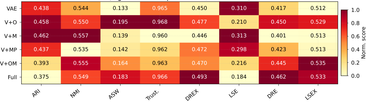
Comprehensive Performance Heatmap (higher = better per column, normalised)
