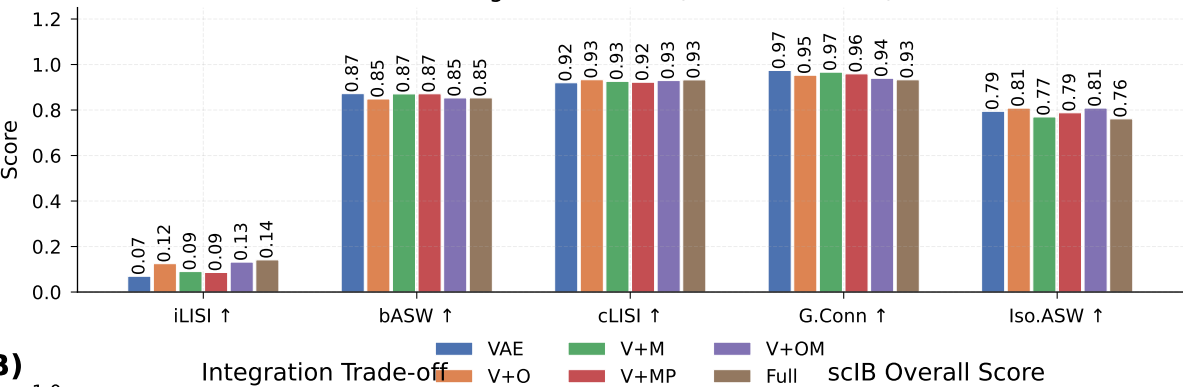
Batch Integration Metrics (IRALL, 8 batches)
