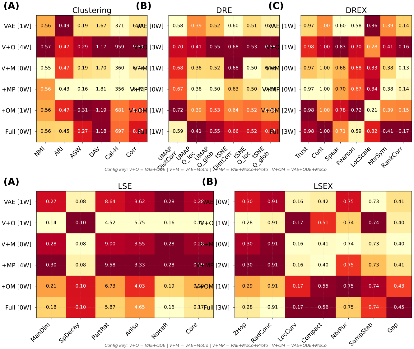
Fig. 11. Subcategory metric breakdown (IRALL, \beta=0.1 , 3,000 cells). Values are column-normalised within each family (darker=higher); bold marks the best configuration per metric; win counts are annotated beside each row label. (A) Clustering (ARI, NMI, ASW, DAV, Cal-H, COR). (B) Dimensionality-reduction evaluation (DRE): latent→UMAP/tSNE fidelity. (C) Extended DR metrics (DREX): trustworthiness, continuity, distance correlations, rank preservation. (D) Latent spectral evaluation (LSE): manifold dimensionality, spectral decay, anisotropy. (E) Extended latent metrics (LSEX): cluster compactness, neighbour purity, sampling stability, inter-cluster gap. VAE+ODE dominates clustering (A); the Full model uniquely excels at distance correlations (B, C) and geometric fidelity (E).
