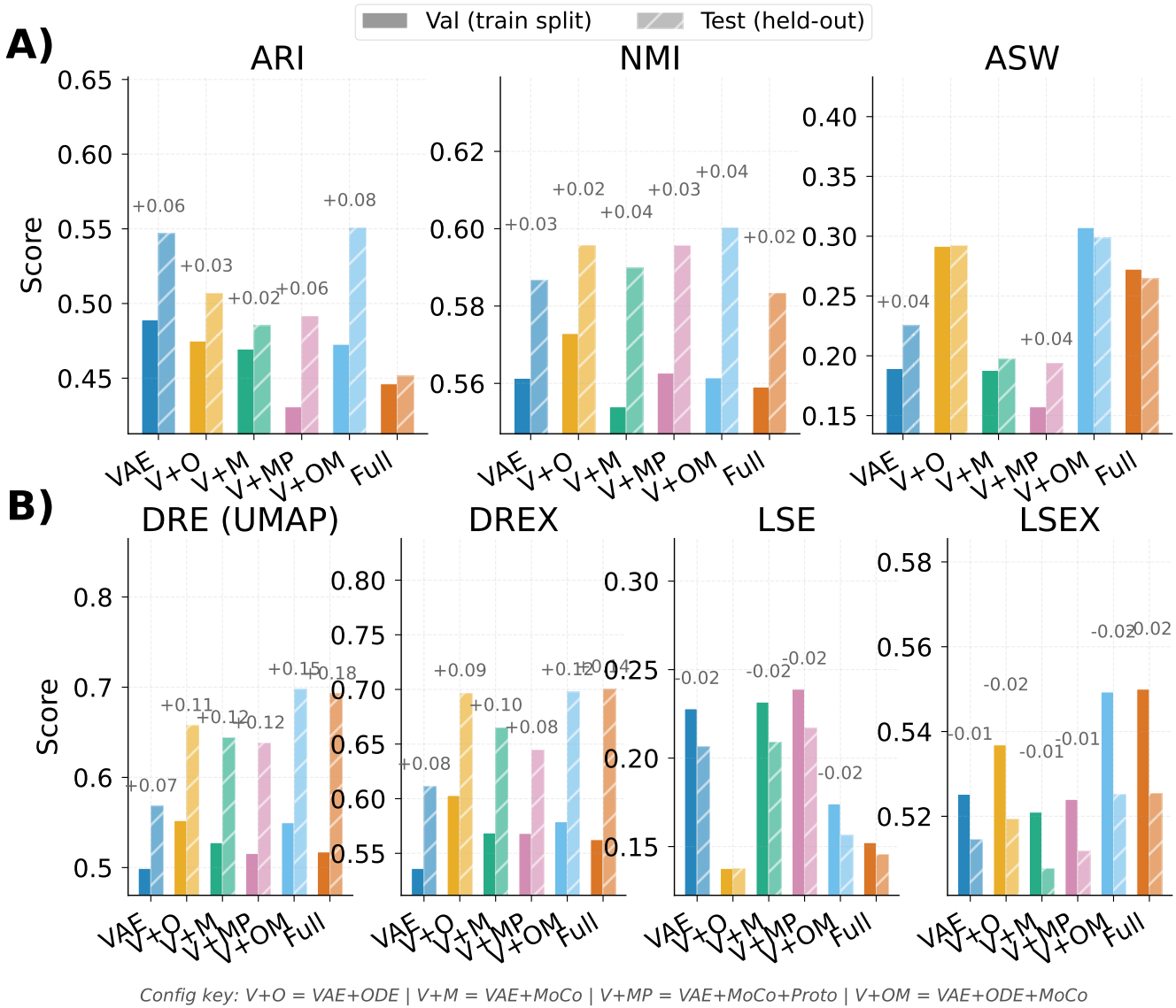
Fig. 7. Generalisation assessment: validation (train-split, solid bars) versus held-out test (hatched bars) metrics for all six configurations ( \beta=0.1 , IRALL). Row 1: Clustering (ARI, NMI, ASW). Row 2: Aggregate quality scores (DRE, DREX, LSE, LSEX). Narrow val-test gaps indicate strong generalisation. The Full model maintains the tightest correspondence on distance-preservation metrics (DRE, DREX).
