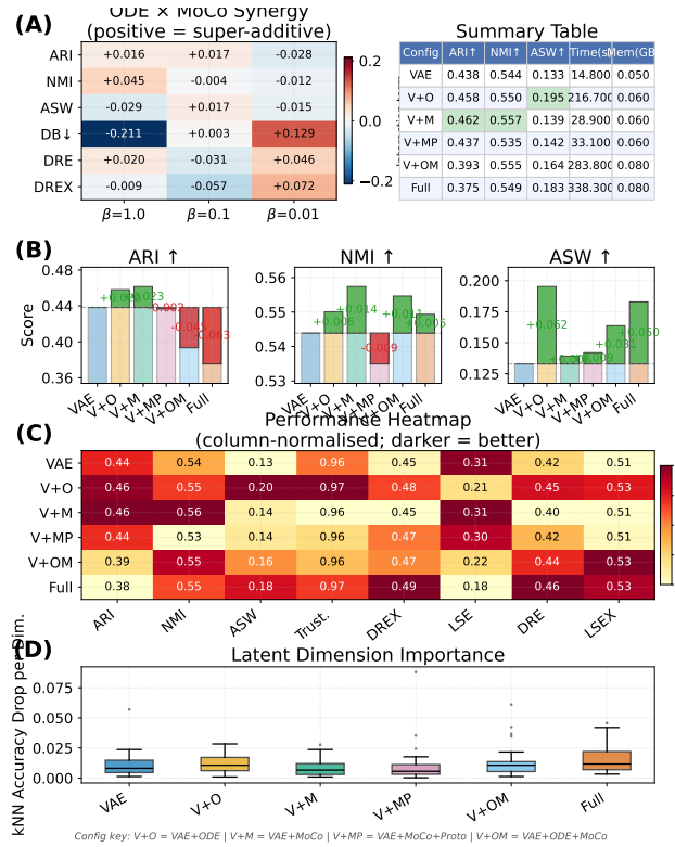
Fig. 3. Component contribution analysis (IRALL, \beta=0.1 ). (A) ODE \times MoCo interaction heatmap across metrics and \beta values; warm tones indicate super-additive effects. (B) Incremental-gain waterfall for ARI, NMI, and ASW: each bar shows the marginal \Delta from the VAE baseline. (C) Column-normalised performance heatmap across eight metrics. (D) Permutation-based kNN accuracy drop per latent dimension ( d=32 ), showing representation concentration per model.
