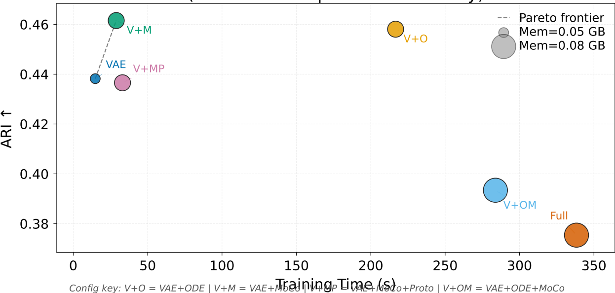
Efficiency: ARI vs Training Time (Bubble size = peak GPU memory)
