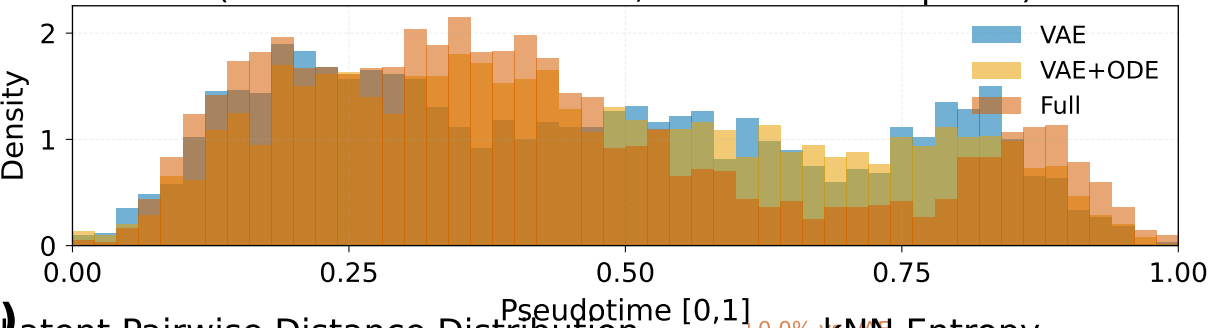
Pseudotime Distribution per Config (ODE latent → smoother, more uniform spread)
