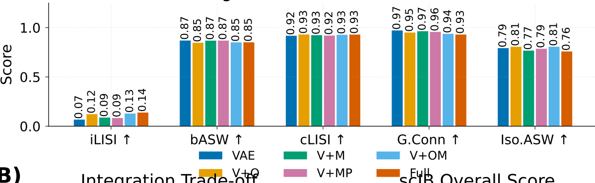
Batch Integration Metrics (IRALL, 8 batches)
