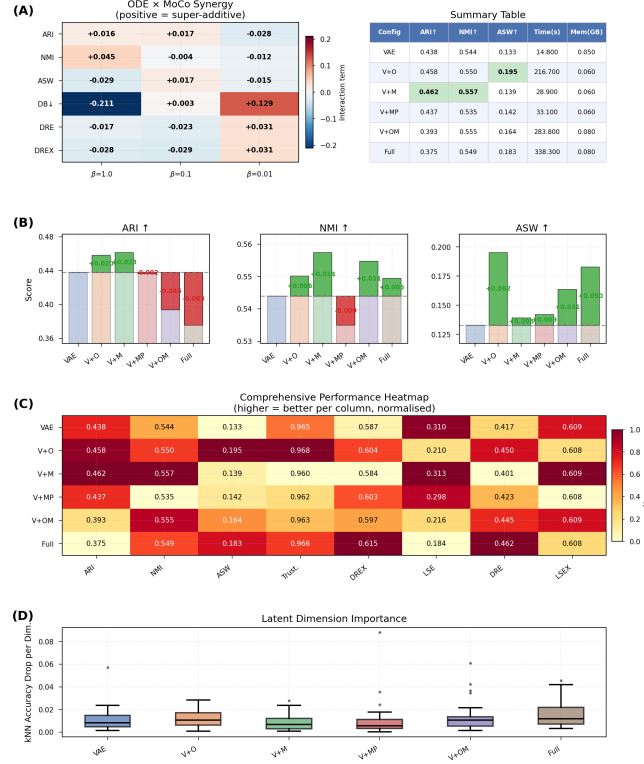
Fig. 3. Ablation study and component contribution analysis (IRALL, \beta=0.1 ). (A) ODE \times MoCo interaction heatmap across metrics and \beta values; warm tones indicate super-additive effects. An adjacent summary table reports key metrics per configuration. (B) Incremental-gain waterfall for ARI, NMI, and ASW: each bar shows the marginal change ( \Delta ) from the VAE baseline (green=positive, red=negative). (C) Column-normalised performance heatmap across eight metrics—no single configuration dominates all axes. (D) Permutation-based kNN accuracy drop per latent dimension ( d=32 ), revealing how concentrated versus distributed each model’s learned representations are.
