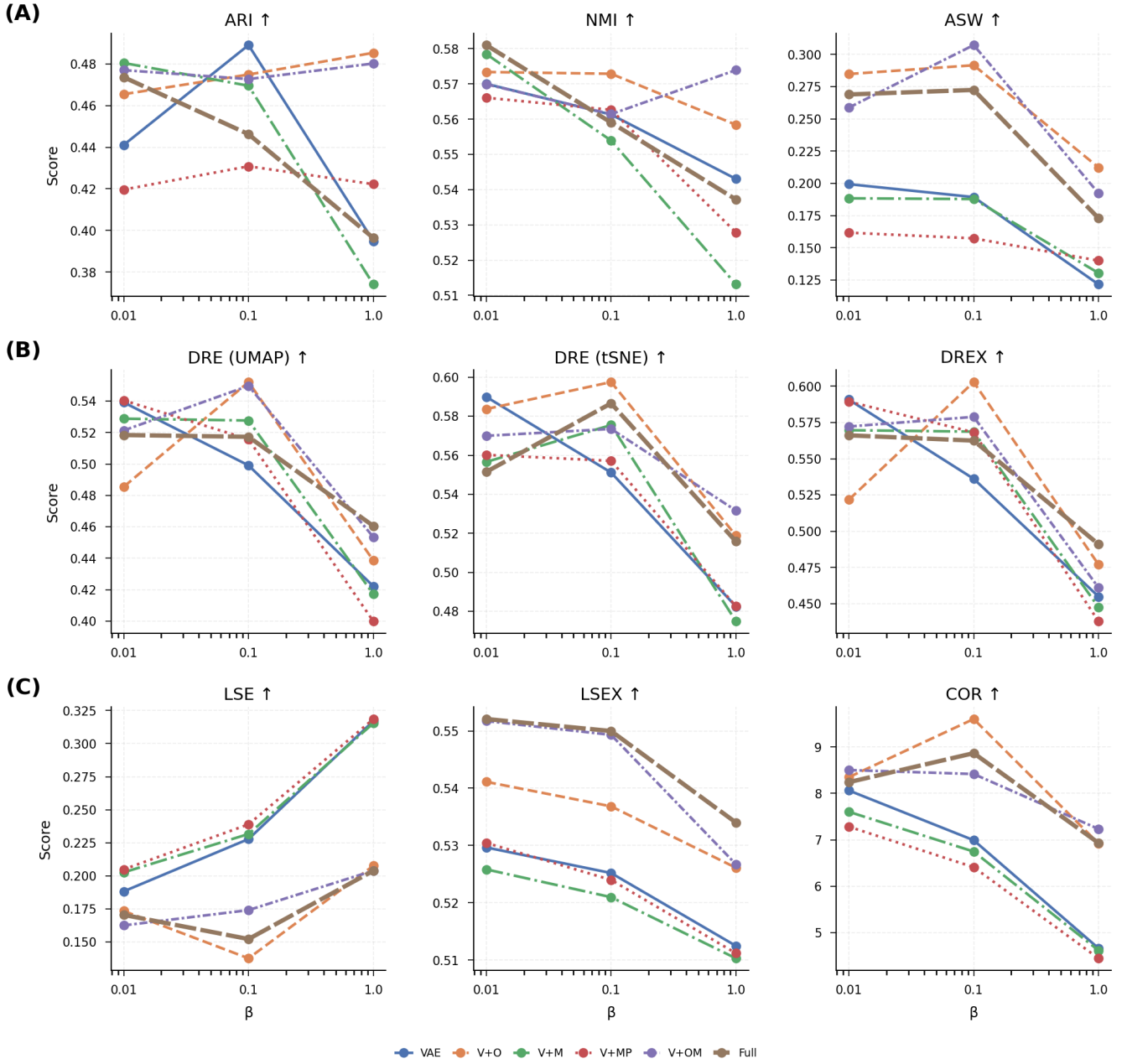
Fig. 7. Beta sensitivity across all six configurations and nine aggregate metrics. Each subplot shows one metric as a function of \beta (log scale, \beta \in \{0.01, 0.1, 1.0\} ), with one line per configuration. ODE-containing models exhibit the most stable profiles; MoCo and prototype effects are strongly \beta -dependent. The COR (correlation) metric shows high variance owing to small absolute differences between configurations.
