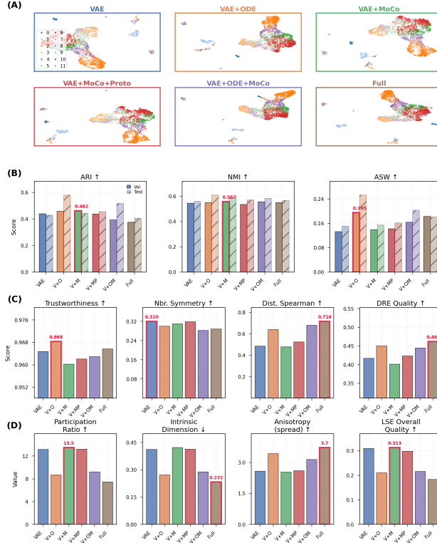
Fig. 2. Quantitative latent-space comparison across six configurations (IRALL, 3,000 cells, 200 epochs, \beta=0.1 ). (A) UMAP projections coloured by cell type show progressive geometric refinement from VAE to Full. (B) Clustering metrics (ARI, NMI, ASW) on validation and held-out test splits; solid and hatched bars respectively. (C) Neighbourhood-preservation metrics (trustworthiness, neighbour symmetry, distance Spearman \rho , DRE). (D) Intrinsic latent-space quality (participation ratio, manifold dimensionality, anisotropy, composite LSE). Bold outlines mark the best configuration per metric.
