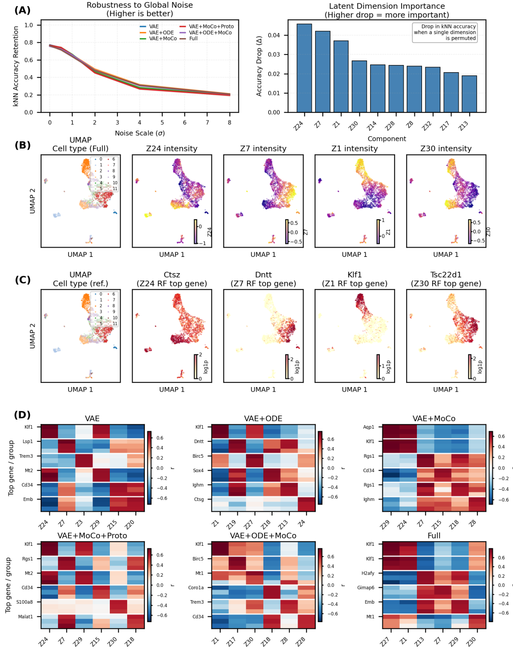
Fig. 11. Biological validation of MoCoO latent spaces (IRALL, Full model). (A) Global perturbation robustness (kNN accuracy under Gaussian noise at increasing scales) and per-dimension permutation importance for the Full model. (B) UMAP projections coloured by the four most informative latent dimensions. (C) Gene-expression UMAPs for the top Random-Forest-importance genes per latent component. (D) Per-configuration Pearson correlation heatmaps between the top genes and top latent components ( 2 \times 3 grid showing all six configurations).
