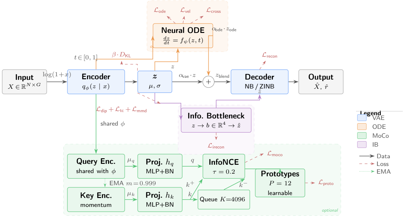
Fig. 1. MoCOO architecture overview. Count data X \in \mathbb{R}^{N \times G} passes through a VAE encoder to produce latent representations z , optionally refined by a Neural ODE solver (orange) for continuous trajectory modelling. Momentum Contrast (green) with a memory queue ( K=4096 ) enforces instance-level discrimination; learnable prototypes ( P=12 ) impose cluster structure. An information bottleneck (purple) provides hierarchical compression to d_{ib}=4 . Dashed regions denote optional modules. Colour coding is consistent throughout all figures.
