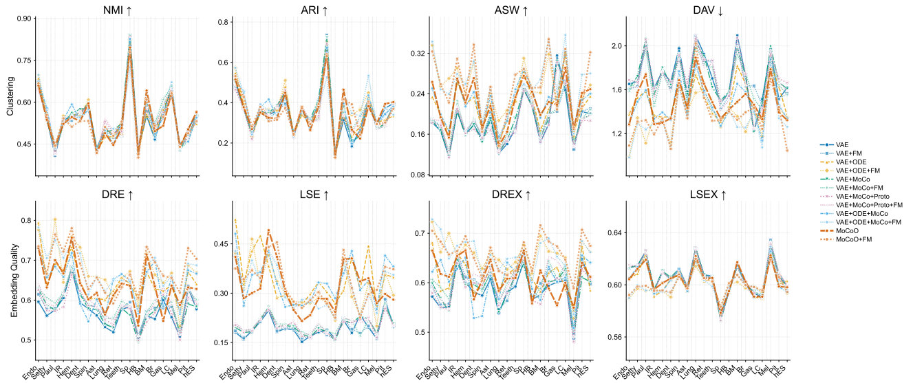
Fig. 7. FM-enhanced per-dataset metric profiles showing all 12 configurations (6 base + 6 FM variants). Each subplot shows one metric across datasets, with FM variants plotted alongside their base counterparts.
