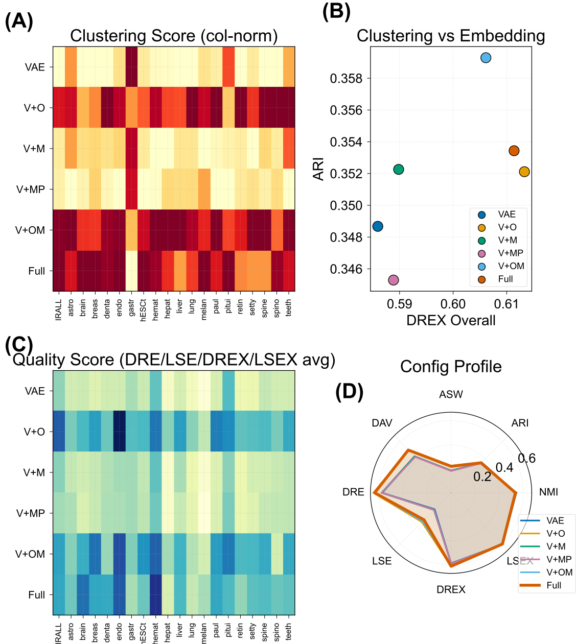
Fig. 10. Cross-dataset evaluation and generalization. (A) Column-normalised clustering-score heatmap (config \times dataset) showing relative ARI performance across all 20 datasets; darker cells indicate stronger performance. (B) ARI vs. DREX scatter (mean across datasets); each point is one configuration—Full (MoCoO) achieves the best DREX–ARI balance. (C) Average embedding quality (DRE, LSE, DREX, LSEX mean) heatmap across all 20 datasets. (D) Radar profile of all eight proposed metrics averaged across datasets; the Full (MoCoO) polygon (thick orange border, filled) covers the largest area, confirming balanced top-tier performance across all metric families.
