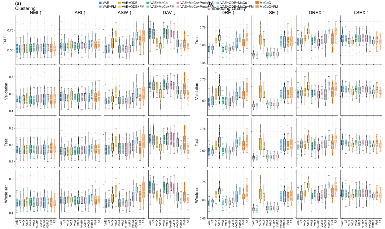
Fig. 4. Flow Matching enhancement across 20 datasets and 12 configurations (6 base + 6 FM-augmented). Each panel compares base versus FM-refined performance on the proposed 8-metric set, revealing which datasets and configurations benefit most from post-training FM refinement. Thick-edged boxes with coloured borders highlight the Full (MoCoO) and MoCoO+FM configurations; notably, Full+FM achieves the outright best DRE and DREX across all 12 configurations (Table VIII).
