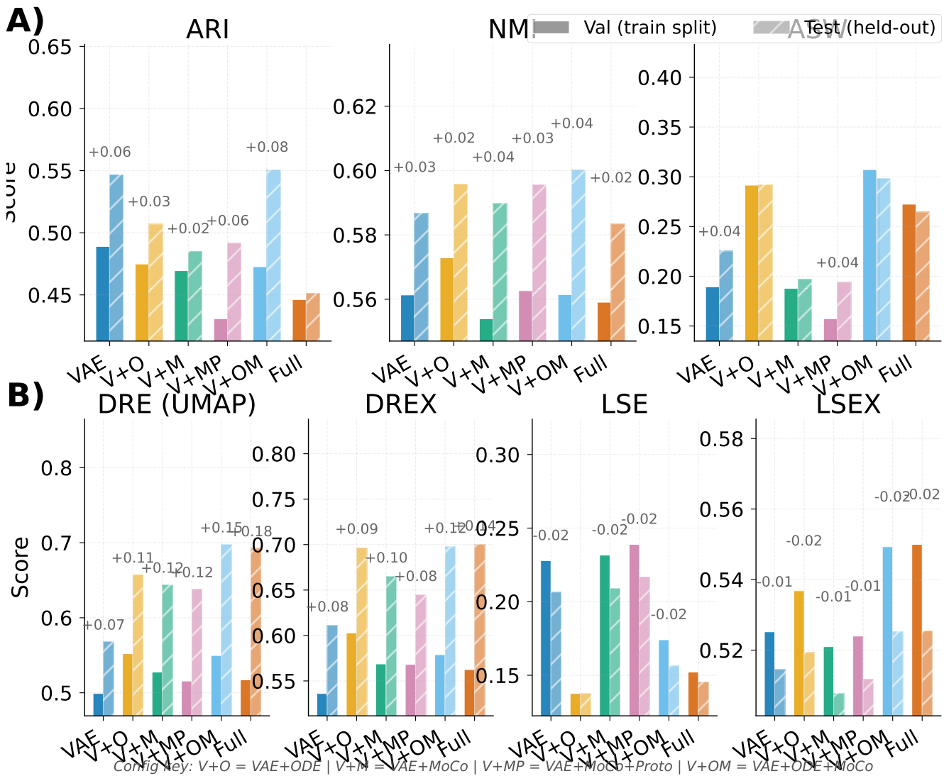
Fig. 7. Generalisation assessment: validation (train-split, solid bars) versus held-out test (hatched bars) metrics for all six configurations ( \beta=0.1 , IRALL). Row 1: Clustering (ARI, NMI, ASW). Row 2: Aggregate quality scores (DRE, DREX, LSE, LSEX). Narrow val-test gaps indicate strong generalisation. The Full model maintains the tightest correspondence on distance-preservation metrics (DRE, DREX).
