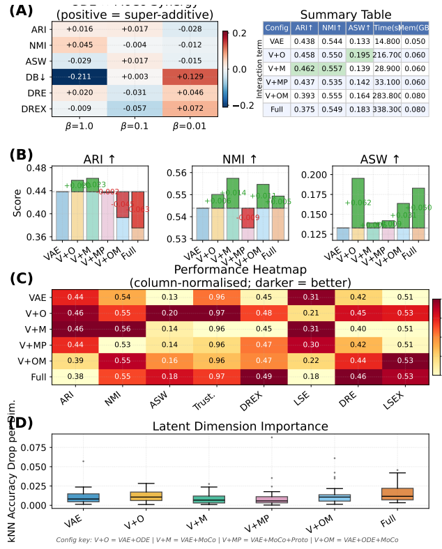
Fig. 3. Component contribution analysis (IRALL, \beta=0.1 ). (A) ODE \times MoCo interaction heatmap across metrics and \beta values; warm tones indicate super-additive effects. (B) Incremental-gain waterfall for ARI, NMI, and ASW: each bar shows the marginal \Delta from the VAE baseline. (C) Column-normalised performance heatmap across eight metrics. (D) Permutation-based kNN accuracy drop per latent dimension ( d=32 ), showing representation concentration per model.
