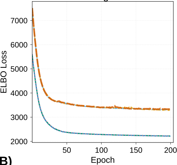
Training Loss
