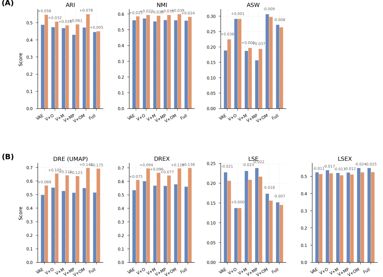
Fig. 8. Generalization assessment: validation (train-split) versus held-out test (test_ext) metrics for all six configurations ( \beta = 0.1 , IRALL). Row 1: Core clustering metrics (ARI, NMI, ASW). Row 2: Aggregate quality scores (DRE, DREX, LSE, LSEX). Smaller val-test gaps indicate better generalization. The Full model maintains the tightest correspondence on distance preservation metrics (DRE, DREX), while all models generalize well on clustering metrics.
