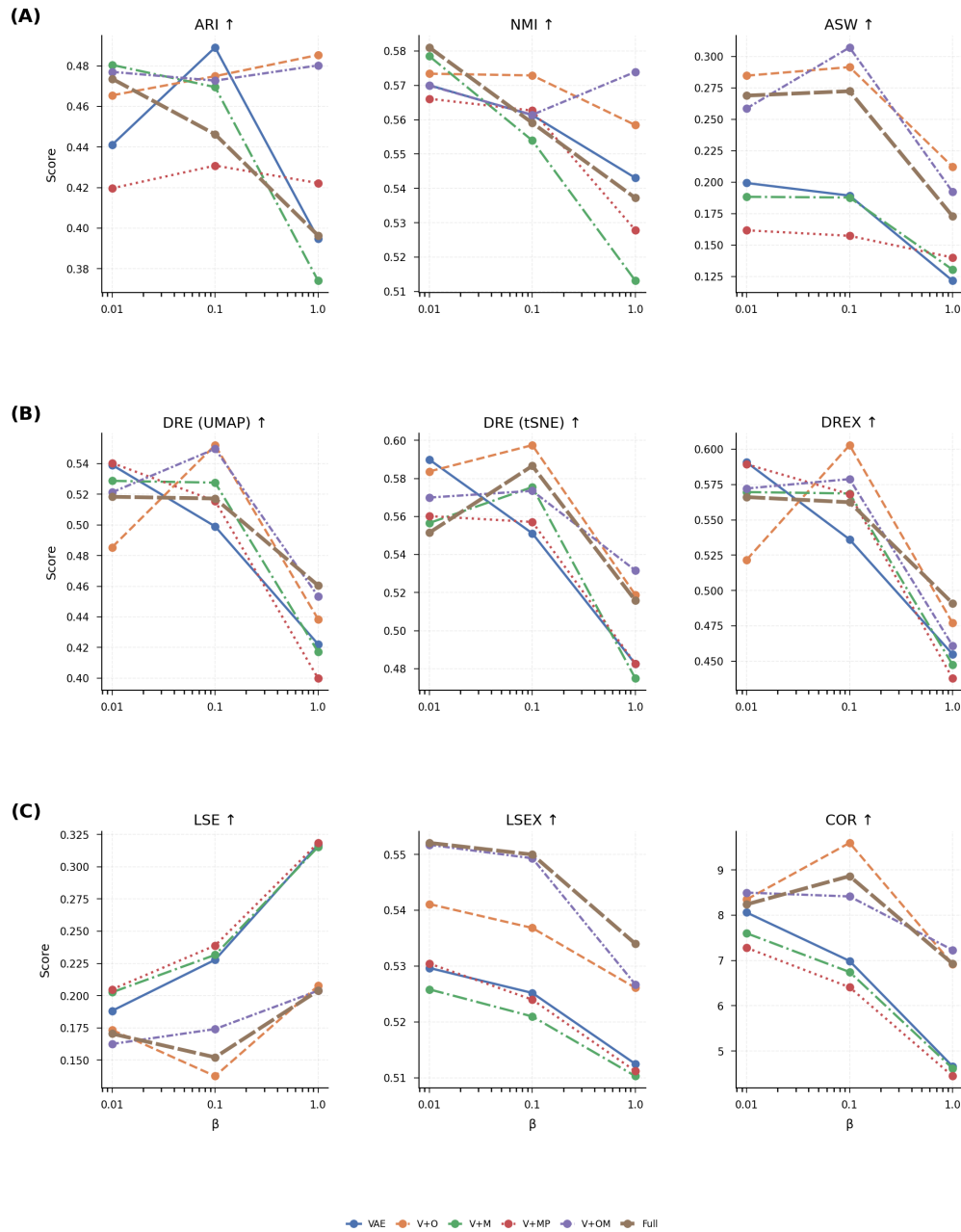
Fig. 7. Beta sensitivity analysis across all six configurations and nine metric families. Each subplot shows one aggregate metric as a function of \beta (log scale), with one line per configuration. ODE-containing models show the most stable profiles across \beta values, while MoCo and Proto effects are strongly beta-dependent. The COR (correlation) metric is included for completeness but shows high variance across configurations.
