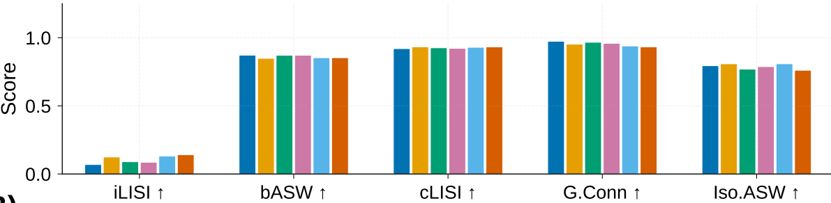
Batch Metrics
