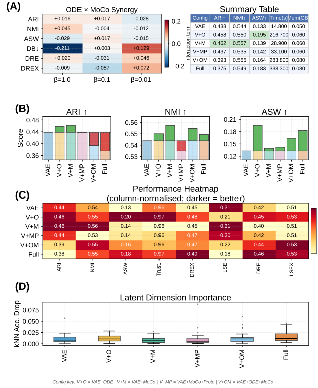
Fig. 3. Component contribution analysis (IRALL, \beta=0.1 ). (A) ODE×MoCo interaction heatmap across metrics and \beta values; warm tones indicate super-additive effects. (B) Incremental-gain waterfall for ARI, NMI, and ASW: each bar shows the marginal \Delta from the VAE baseline. (C) Column-normalised performance heatmap across eight metrics. (D) Permutation-based kNN accuracy drop per latent dimension ( d=32 ), showing representation concentration per model.
