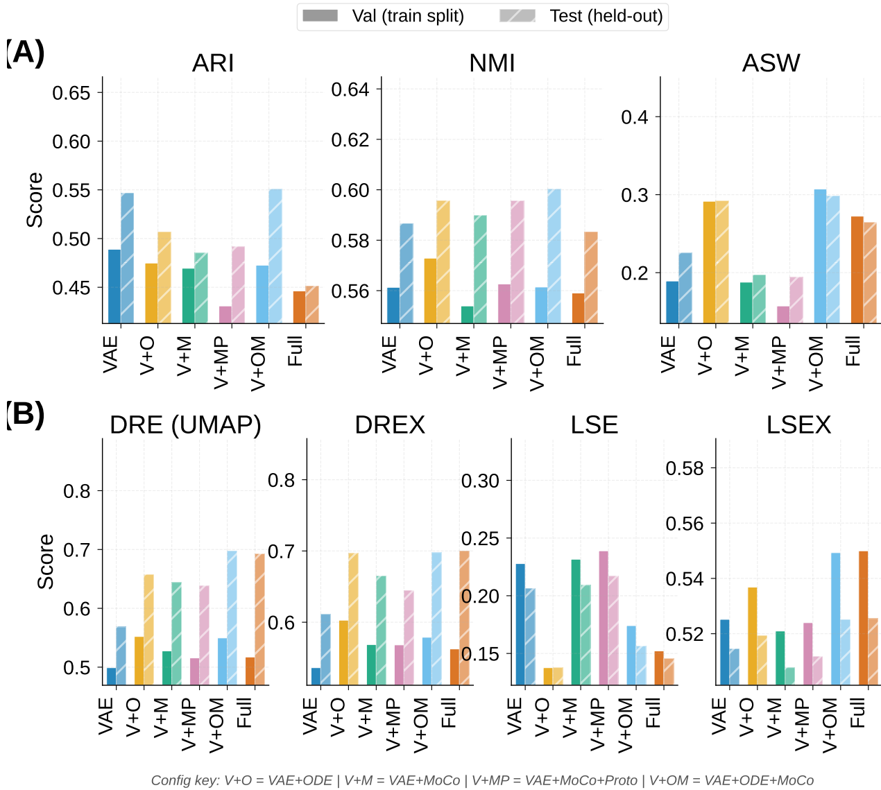
Fig. 7. Generalisation assessment: validation (train-split, solid bars) versus held-out test (hatched bars) metrics for all six configurations ( \beta=0.1 , IRALL). Row 1: Clustering (ARI, NMI, ASW). Row 2: Aggregate quality scores (DRE, DREX, LSE, LSEX). Narrow val-test gaps indicate strong generalisation. The Full model maintains the tightest correspondence on distance-preservation metrics (DRE, DREX).
