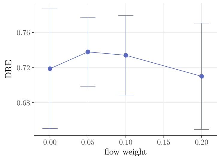
Flow weight: DRE-UMAP
