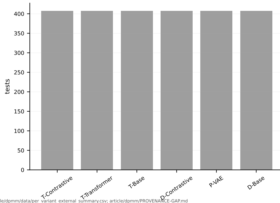
Test-count coverage
