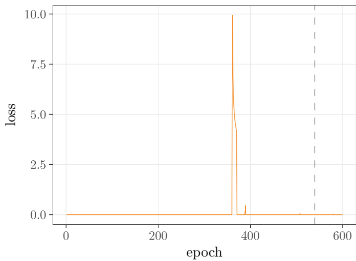
DPMM loss after warmup
