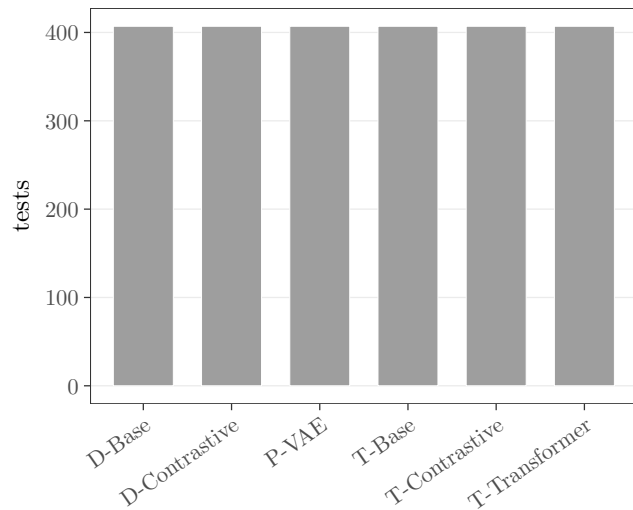
Test-count coverage
