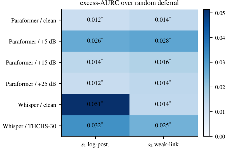
Figure 6: Realized m=12 audit family: excess-AURC over analytic random deferral for \{s_1, s_2\} across six (backbone \times condition) cells. Cell magnitudes are the informative quantity; their speaker-blocked bootstrap 95% CIs (all excluding zero) are in table 5. The * marks the permutation rejection, which is saturated at the floor for every cell ( p_{\text{Holm}}=0.006 ) and hence non-discriminating.
