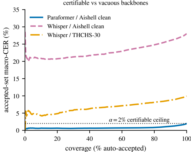
Figure 5: Why the certificate is vacuous on weak backbones. Paraformer/Aishell dips below the \alpha=2\% ceiling (certifiable); Whisper/Aishell and Whisper/THCHS-30 plateau far above it, so no threshold yields a \leq 2\% accepted set — even though the audit still finds significant selective skill on these backbones.
