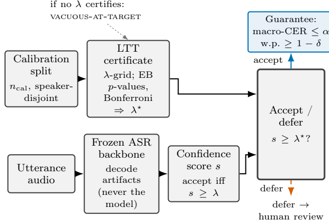
Figure 1: The asr-gate pipeline. Decode artifacts from a frozen ASR backbone (never the model itself) yield a per-utterance confidence score s (e.g. s_1, s_2 ); a speaker-disjoint calibration split ( n_{\text{cal}} ) drives Learn-Then-Test (3) construction of a threshold \lambda^* (the frozen EB- p -value, Bonferroni-over-grid procedure of section 2.2) certifying, with probability at least 1 - \delta , that the accepted set’s macro-CER does not exceed \alpha ; each utterance is then accepted ( s \geq \lambda^* ) or deferred to a human. If no threshold on the grid certifies, the gate reports VACUOUS-AT-TARGET rather than accepting nothing silently.
