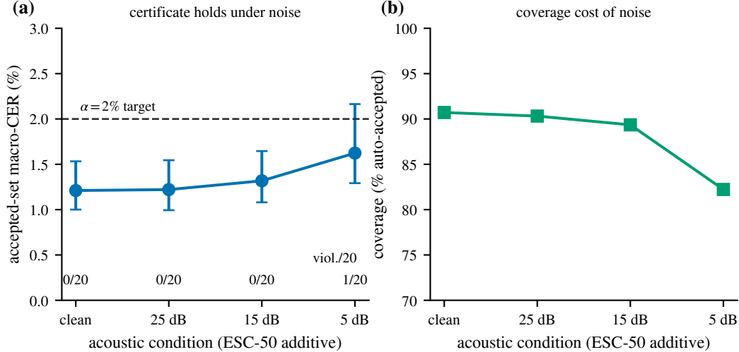
Figure 5: Noise robustness: the clean-calibrated Paraformer gate applied to ESC-50 additive noise. (a) Accepted-set macro-CER (error bars: min-max over 20 reseeds) stays under the \alpha=2\% target with 0/20 violations at 25 and 15 dB and 1/20 at 5 dB (within the \delta=0.1 budget). (b) Coverage cost of noise: mean auto-accepted fraction falls from 90.7% on clean audio to 90.3%/89.4% at 25/15 dB and 82.2% at 5 dB.
