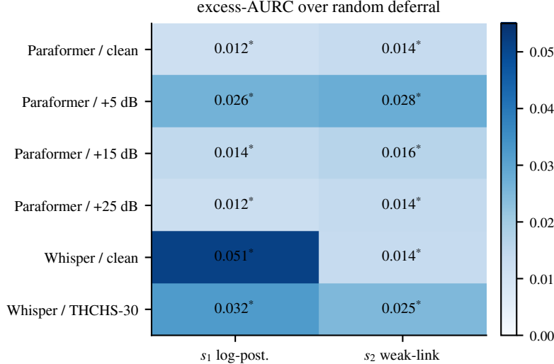
Figure 7: Realized m=12 audit family: excess-AURC over analytic random deferral for \{s_1, s_2\} across six (backbone \times condition) cells. Cell magnitudes are the informative quantity; their speaker-blocked bootstrap 95% CIs all exclude zero (Holm-controlled audit family). The * marks the permutation rejection, which is saturated at the floor for every cell ( p_{\text{Holm}}=0.006 ) and hence non-discriminating.
