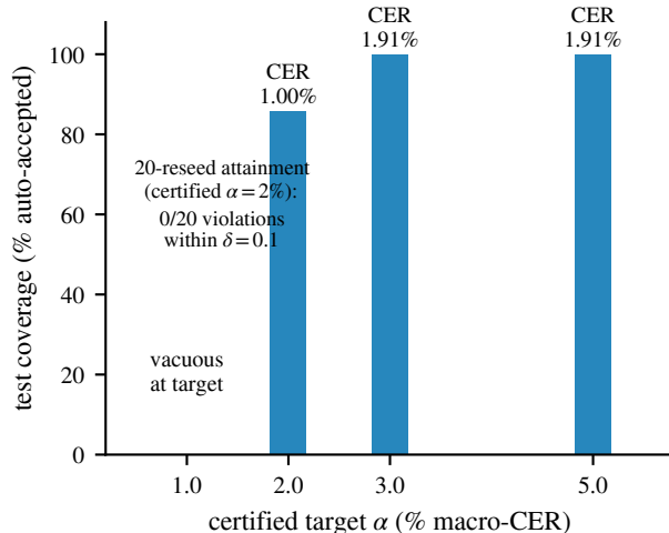
Figure 3: Certified frontier (Paraformer test), at reference reseed 0 (the minimum-acceptance reseed; the 20-reseed mean acceptance at \alpha=2\% is 90.7%). \alpha=1\% is VACUOUS-AT-TARGET (0% acceptance); \alpha=2\% certifies at 85.7% coverage; \alpha=3\% and 5\% saturate at 99.8%. The annotation over the vacuous \alpha=1\% column reports the \alpha=2\% certificate’s reseed attainment: 0/20 violations across the 20 reseeds, within the \delta=0.1 budget.
