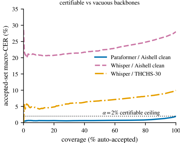
Figure 6: Why the certificate is vacuous on weak backbones. Paraformer/Aishell dips below the \alpha=2\% ceiling (certifiable); Whisper/Aishell and Whisper/THCHS-30 plateau far above it, so no threshold yields a \leq 2\% accepted set — even though the audit still finds significant selective skill on these backbones.
