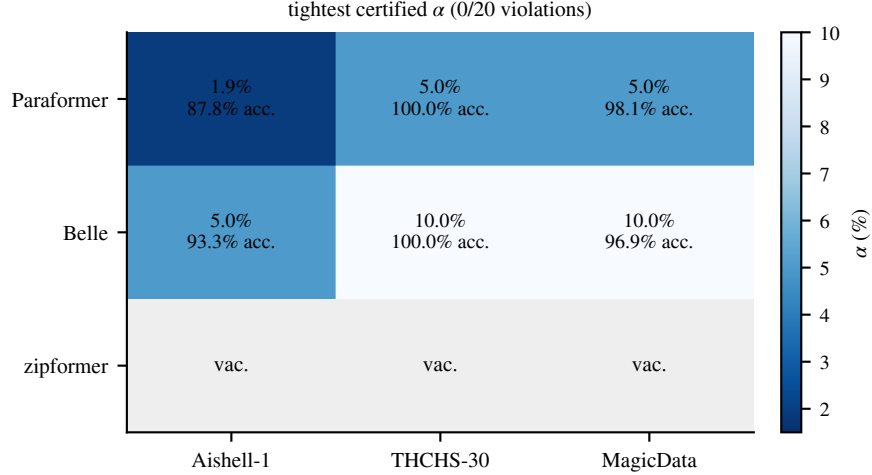
Figure 8: Certified landscape: tightest non-vacuous target (20 reseeds, 0 violations) for three backbones \times three Mandarin corpora. Cell text is that target and mean acceptance. Vacuous cells accept nothing. Paraformer/Aishell-1 uses the binding 1.9% target; other cells use the frozen \alpha -grid.
