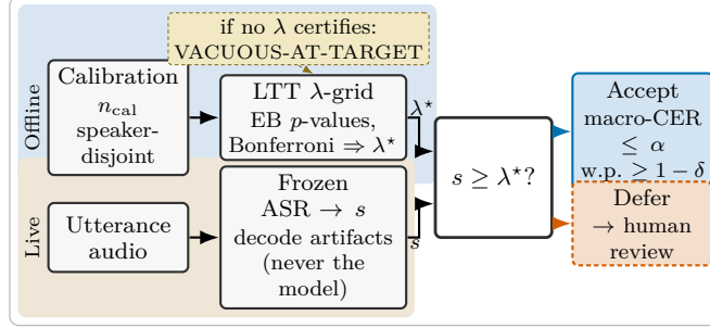
Figure 1: Certified transcription-triage pipeline. Decode artifacts from a frozen ASR backbone (never the model itself) yield a per-utterance confidence score s (e.g. s_1, s_2 ); a speaker-disjoint calibration split ( n_{cal} ) drives Learn-Then-Test construction of a threshold \lambda^* (empirical-Bernstein p -values with a Bonferroni-over-grid selective-risk procedure) certifying, with probability at least 1 - \delta , that the accepted set’s macro-CER does not exceed \alpha ; each utterance is then accepted ( s \geq \lambda^* ) or deferred to a human. If no threshold on the grid certifies, the gate reports VACUOUS-AT-TARGET rather than accepting nothing silently.
