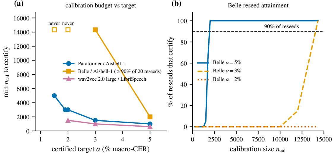
Figure 4: Calibration budget versus certified target, from archived calibration-size records (no new decoding). (a) Smallest n_{\text{cal}} at which the accept/defer gate certifies non-vacuously: Paraformer and Belle on Aishell-1, and wav2vec 2.0 large on LibriSpeech. Open markers sit at the available pool when that target never certifies. (b) Belle: fraction of 20 calibration reseeds that certify at \alpha = 5\% , 3\% , and 2\% . The dashed line at 90\% is the stability cutoff for the smallest reported n_{\text{cal}} .
