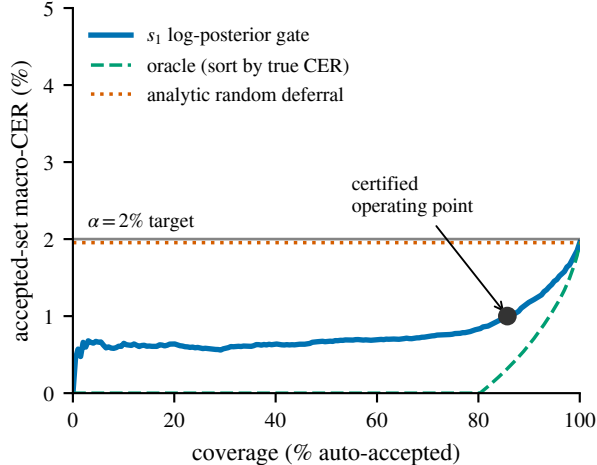
Figure 2: Risk-coverage on Aishell-1 test (Paraformer, s_1 ): the confidence gate (blue) tracks well below the analytic random-deferral line (dotted) and approaches the oracle (dashed). The marked operating point is reference reseed 0 (the minimum-acceptance reseed): it auto-accepts 85.7% of utterances at 1.00% macro-CER, under the \alpha=2\% target; the mean over 20 reseeds is 90.7% acceptance. (The dotted random-deferral asymptote is the s_1 -audit-subset macro-CER, 1.95% over the n=7,172 utterances with a non-null s_1 ; the 1.98% full-set figure (The dotted random-deferral asymptote is the s_1 -audit-subset macro-CER, 1.95% over the n=7,172 utterances with a non-null s_1 ; the full-set macro-CER 1.98% is over all n=7,176 utterances — hence the 1.95 vs 1.98% hair.)
