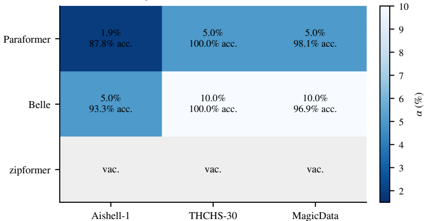
tightest certified \alpha (0/20 violations)
